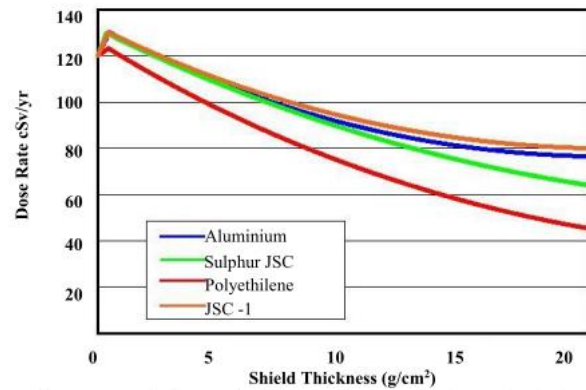
Figure 4. Sulfur concrete, aluminum, polyethylene and lunar regolith (JSC-1 simulant) on radiation test graphic
