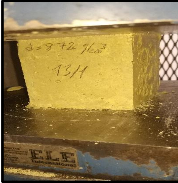
Figure 8. Sample During Test
