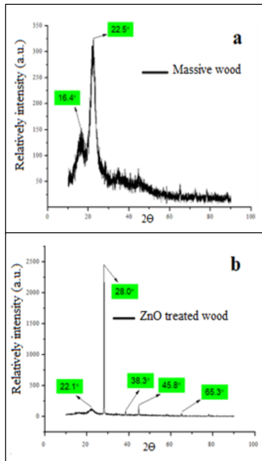
Figure 4. XRD spectrum of (a) solid wood (b) ZnO interfered wood
