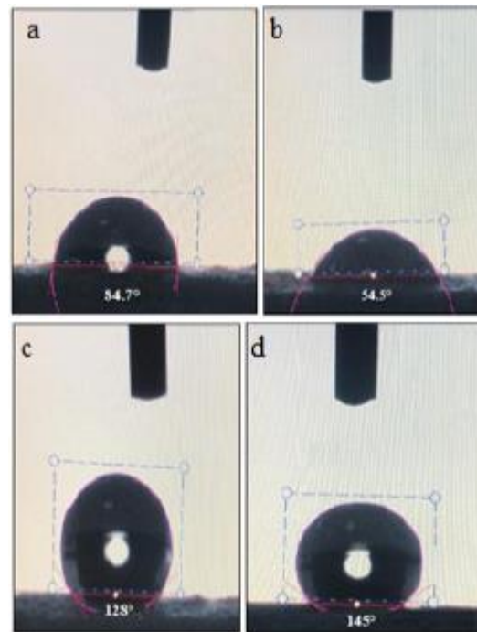
Figure 6. untreated wood (a), ZnO treated wood (b), FAS-17 treated wood (c) and (d) ZnO and FAS-17 treated wood.
