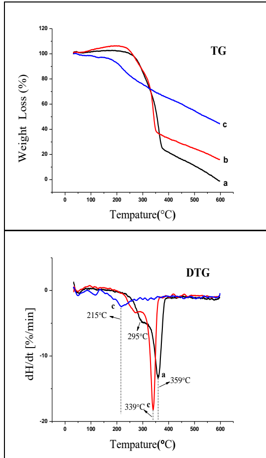
Figure 5. Thermal analysis (TG/DTG) profile (a) solid wood; (b) ZnO interfered wood (c) ZnO-treated wood hydrophobization with FAS-17.
