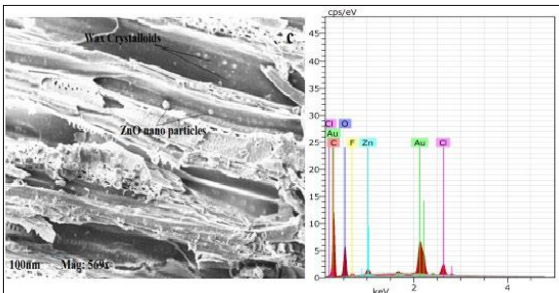
Figure 7. SEM images and EDX spectrum of (a) Massive wood, (b) Massive-ZnO and (c) Massive-ZnO@FAS-17.
