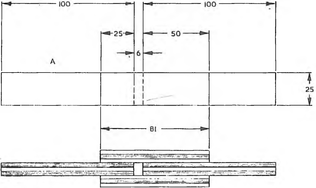
Şekil 1 : Dönme-makaslama test örneği (B.S. 4512'den) Figure 1 : Rolling shear test specimen (From B.S. 4512)
