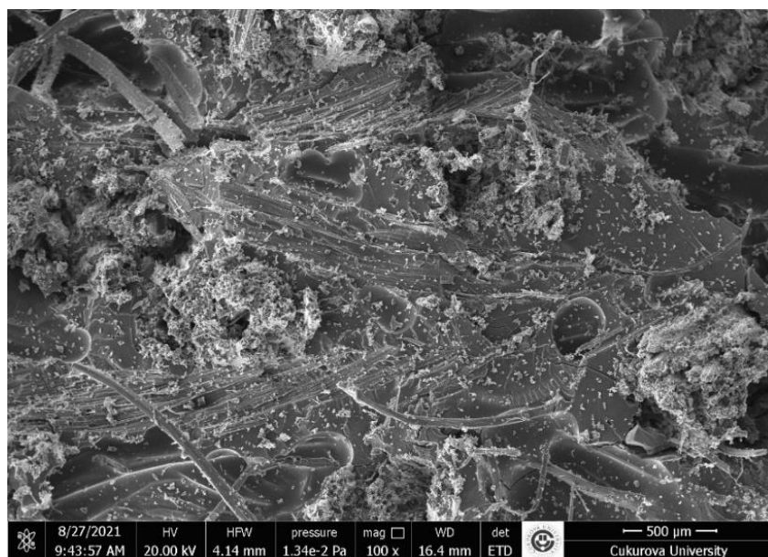
Fig. 16. Morphological images of J sample at 80 °C post-cure temperature
