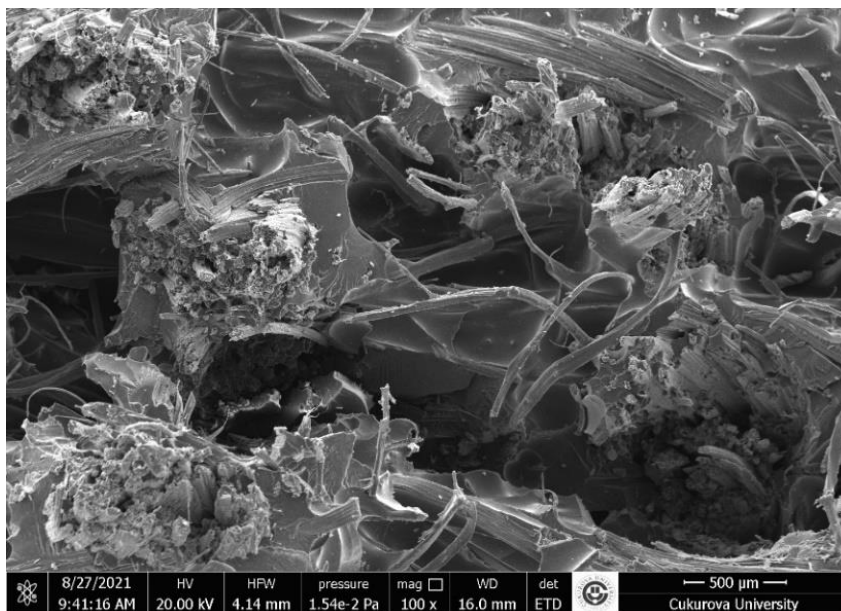
Fig. 15. Morphological images of J sample at 60 °C post-cure temperature
