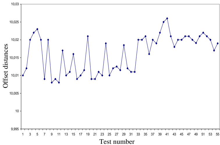
Figure 5. Offsets of the X and Z axis resultant according to the tests number
