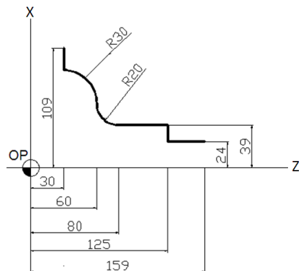
Figure 10. Example of a machining program
