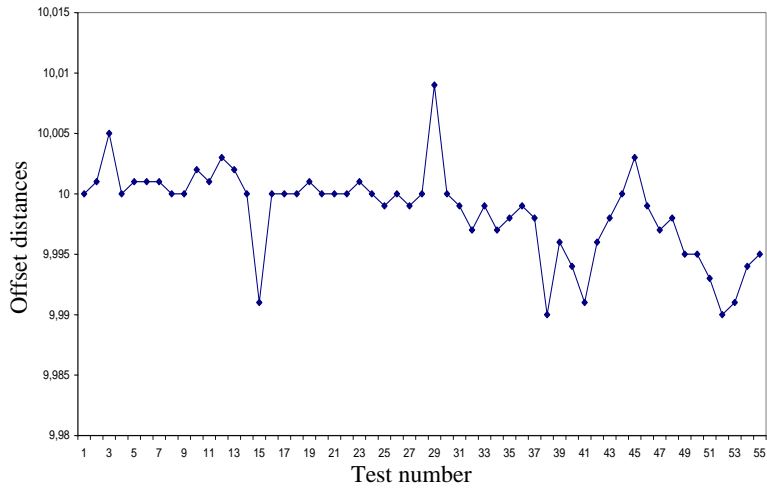
Figure 4. Z axis Offsets according to the tests number
