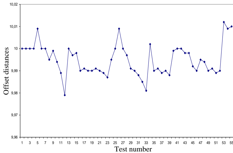
Figure 3. X axis Offsets according to the tests number
