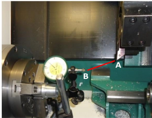
Figure 6. Offset by the interpolation of (X Z)
