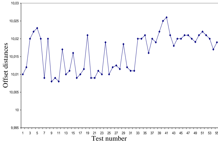
Figure 7. X and Z axis Offsets according to the tests number
