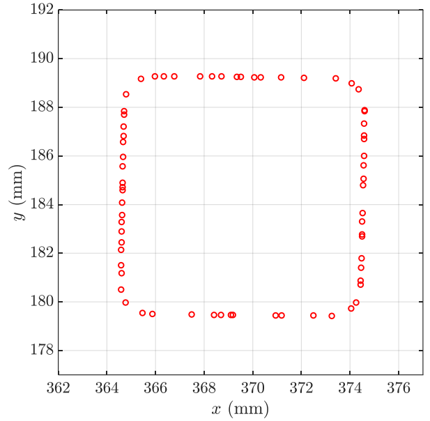
Fig. 2 Example CMM measurement
