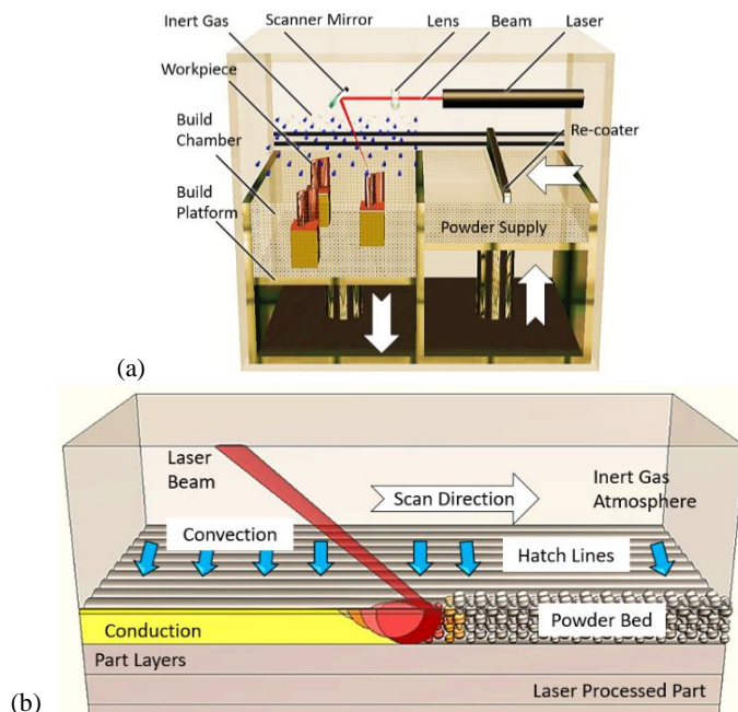
Figure 1. (a) Schematics of laser powder bed fusion AM; (b) heat transfer mechanisms occur as the result of process.
