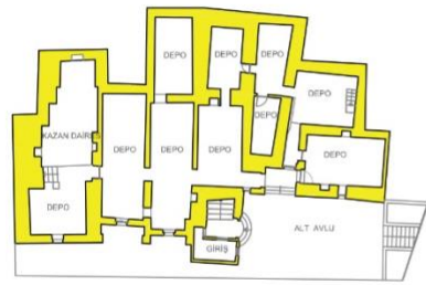
BODRUM KAT PLANI
