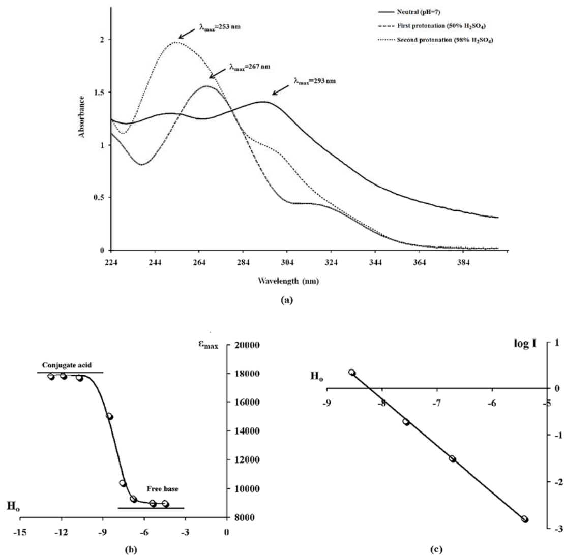
Figure 2. (a) Absorption spectra at different acidity range, (b) \epsilon_{\max} as a function of H_0 and (c) H_0 as a function of \log I of compound 2
