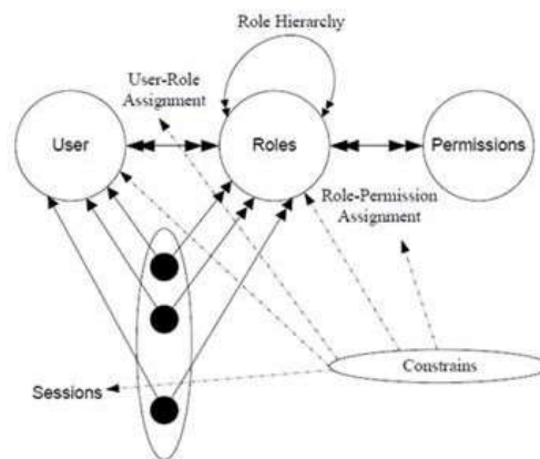
Figure 1. Role-Based Access Control Model (Lu et al. 2017)
