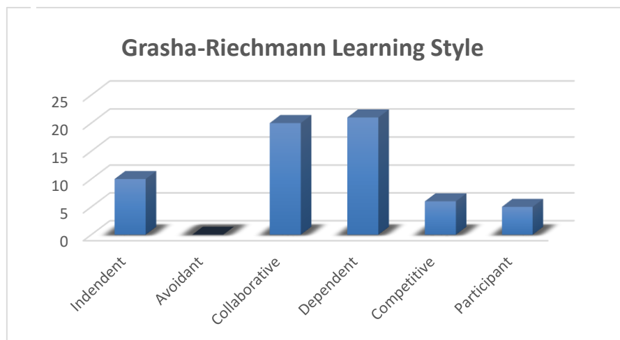
Figure 2. Learning
