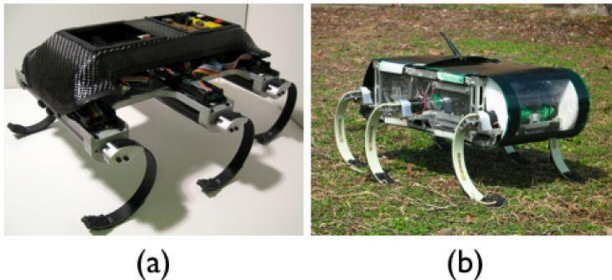
Fig. 1. (a) EduBot (b) RHex platforms.
