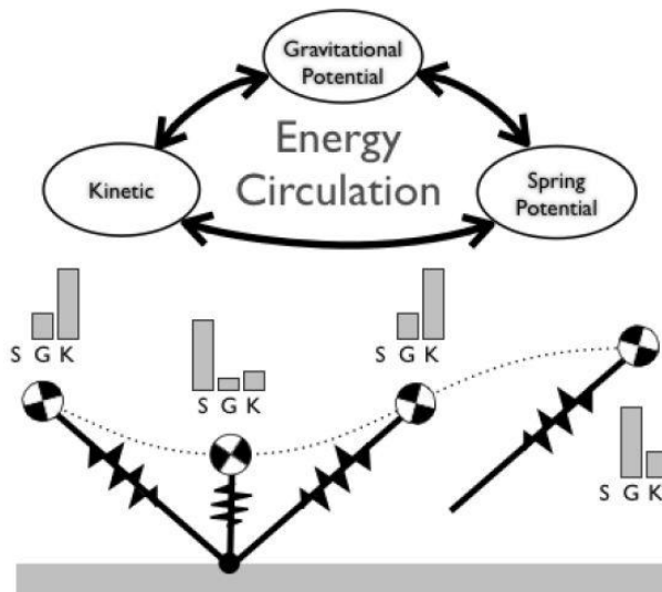
Fig. 4. Energy circulation in the spring loaded inverted pendulum (SLIP) model. The top illustration indicates the major forms of energy in the system and pathways for exchange. The bottom illustration captures four states of a SLIP stride and the distribution of total energy among the three forms of energy. SLIP system alternately uses the gravitational and elastic potential energy to store energy and redirect it to kinetic energy.
