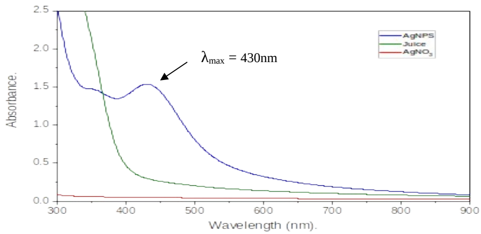
Figure 3: UV-Visible spectra of AgNPs from lemon juice.
