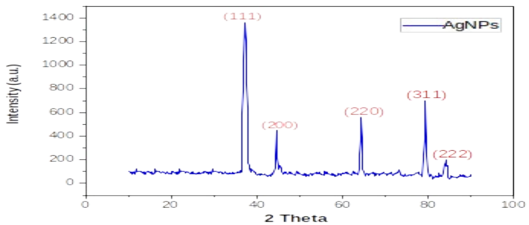
Figure 5 : XRD-spectrum of AgNPs synthesized.
