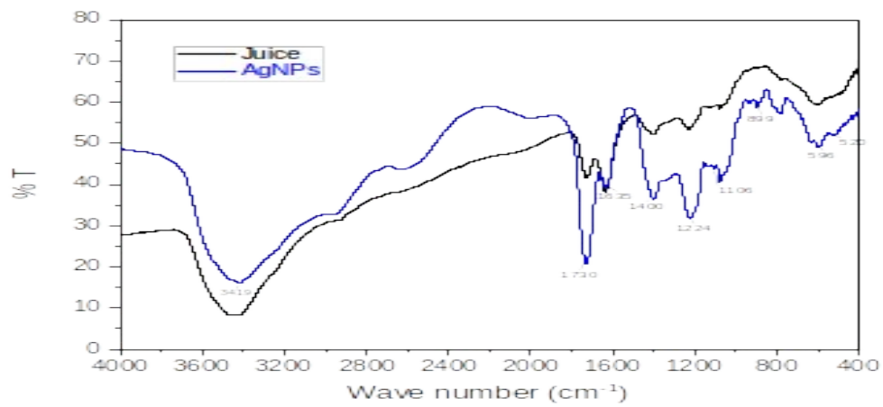
Figure 4 :- FT-IR spectra of lemon juice and AgNPs .
