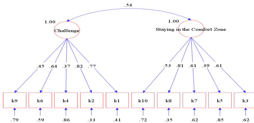
Figure 3 CFA Diagram Regarding the Comfort Zone Orientation Scale
