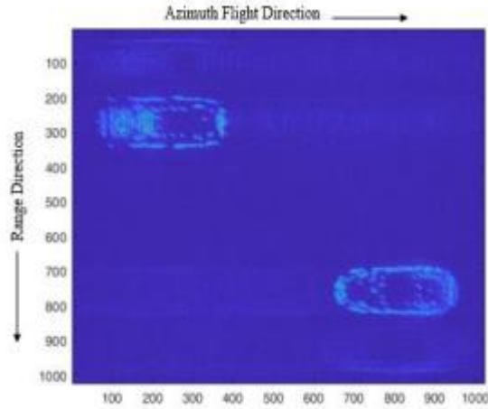
Figure 3. PFA image of Honda and Toyota CAD model stationary targets
