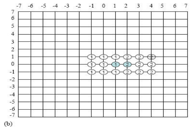
Fig. 6. (a), (b) Examples to illustrate the MGDS algorithm (Huang & Tsai, 2004)
