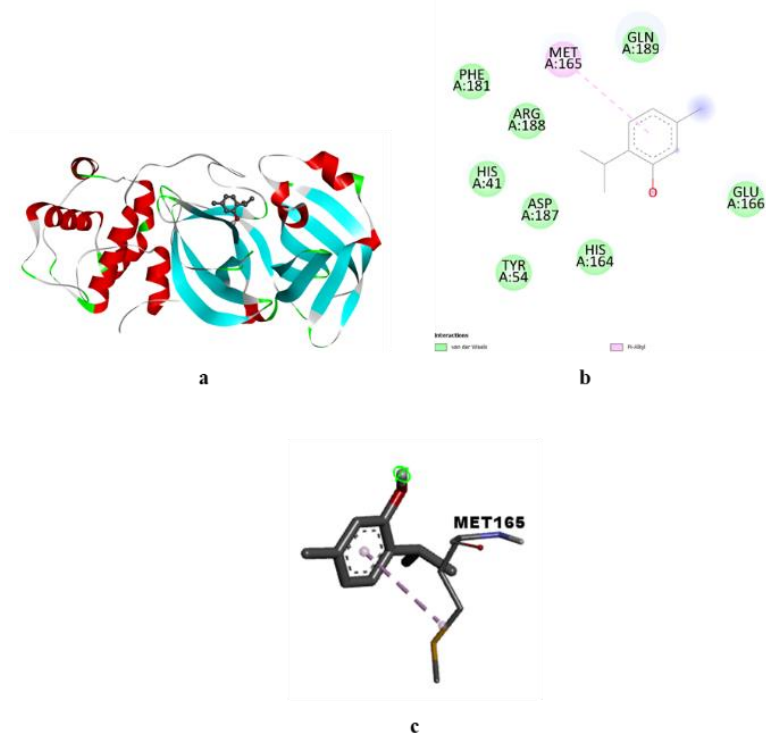
Figure 2. The Molecular docking results of thymol on the MPro enzyme (a), 2D interactions of thymol with the active region of the MPro enzyme (b), and ligand interactions between thymol and the active region of the MPro enzyme (c).
