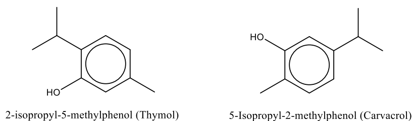
Figure 1. Structures of thymol and carvacrol.
