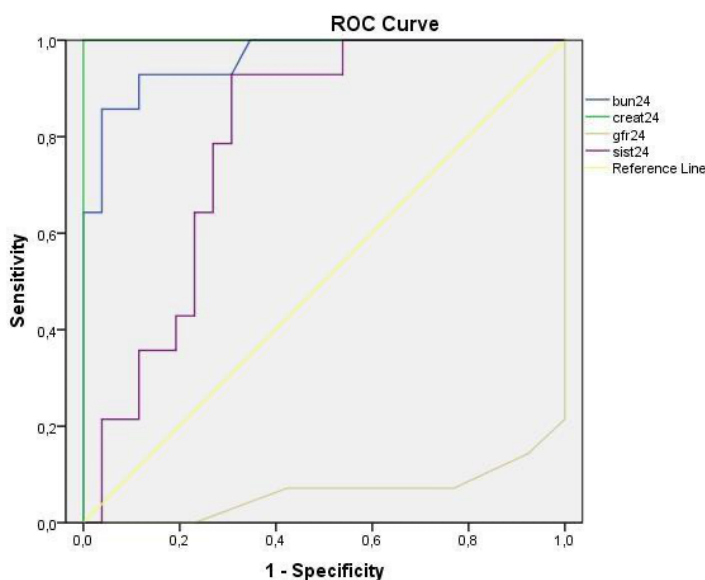
Figure 1. 24-hour ROC analysis result according to AKIN classification
