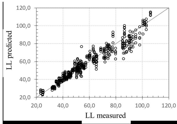
Figure 6. Comparison between the predicted liquid limits versus the measured liquid limits.
