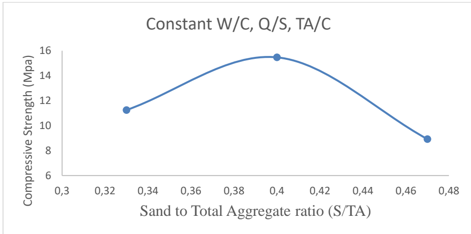
Fig. 1 Relationship between S/TA and 28 day compressive strength
