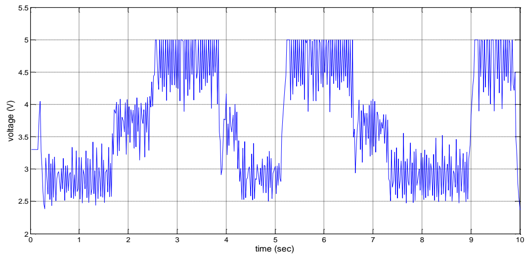
Figure 12: FLC signal output against dc motor load change (no-loaded, half, and full loaded).
