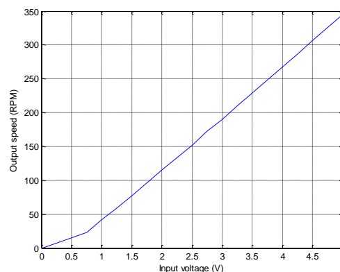
Figure 10: DC motor input-output relationship.
