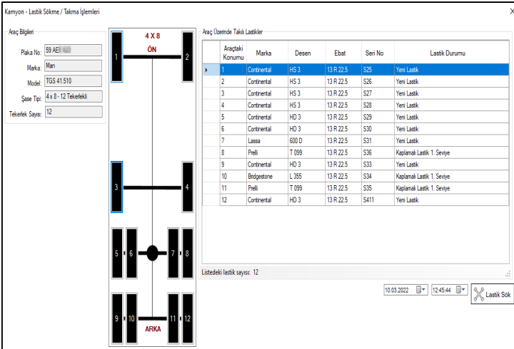
Figure 8. Tire Removal/Assembly Operations
