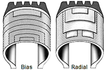
Figure 2. Bias and radial tires
