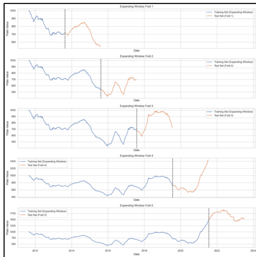
Figure 2. Expanding window cross – validation.
