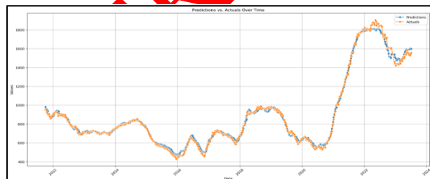
Figure 7. Forecast plot of entire dataset by GRU
