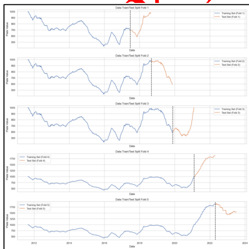
Figure 3. Time series cross – validation
