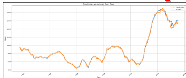
Figure 6. Forecast plot of entire dataset by LSTM
