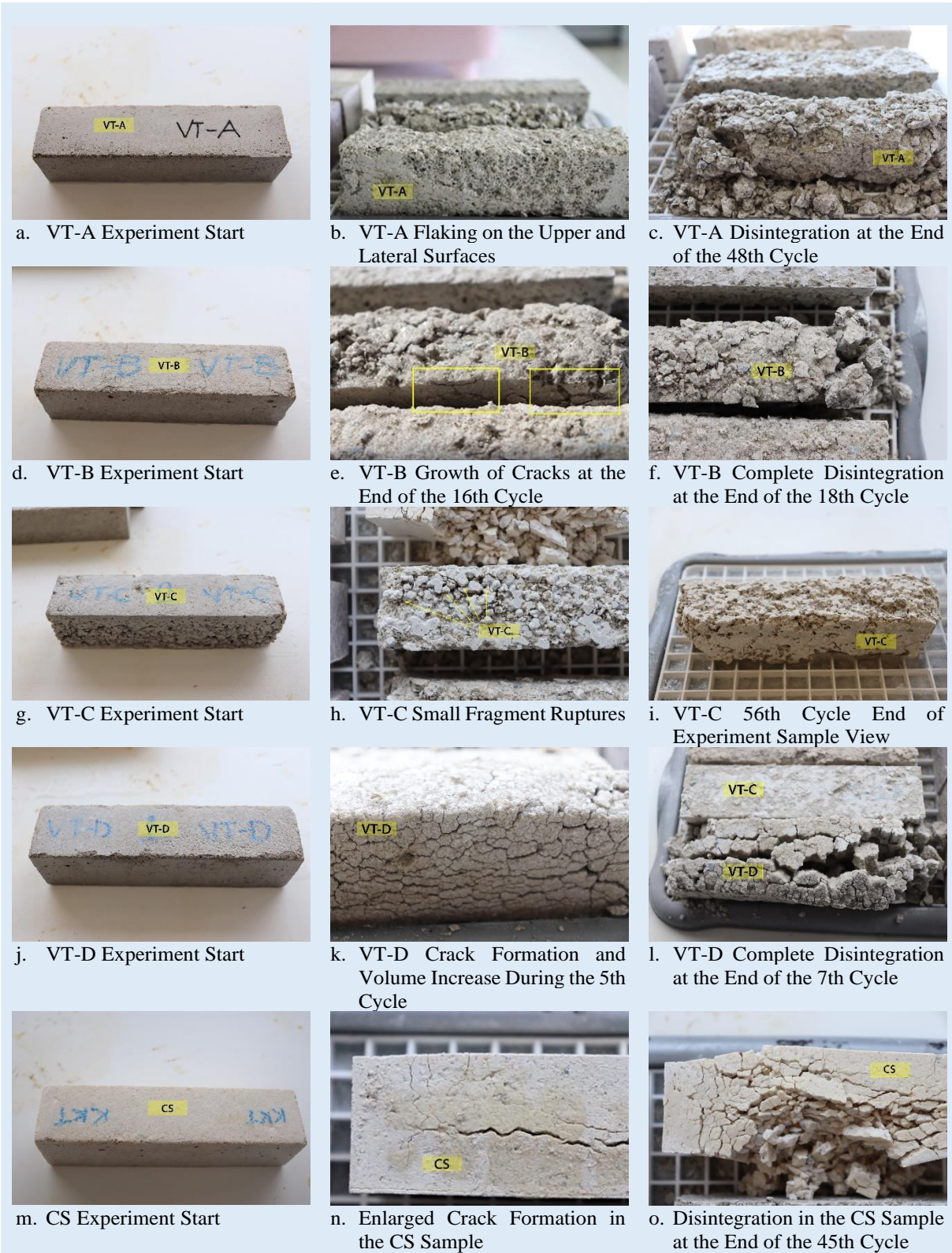
Figure 4. Freeze-Thaw Effects on Samples
