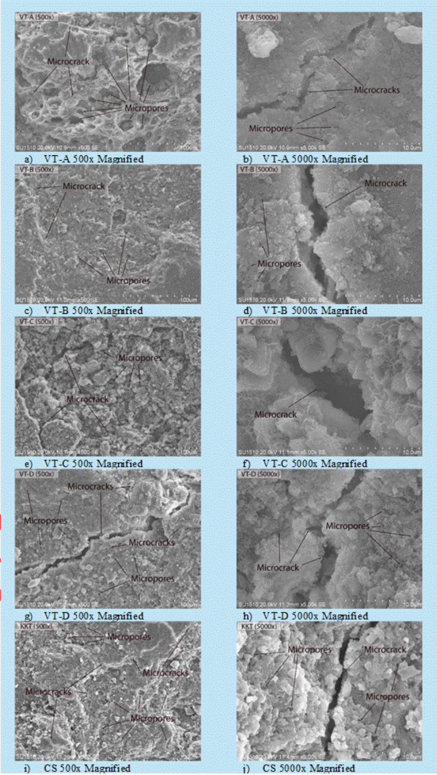
Figure 5. SEM Images at 500x and 5000x Magnification
