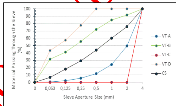
Figure 3. Aggregate Granulometries of the Sample Types
