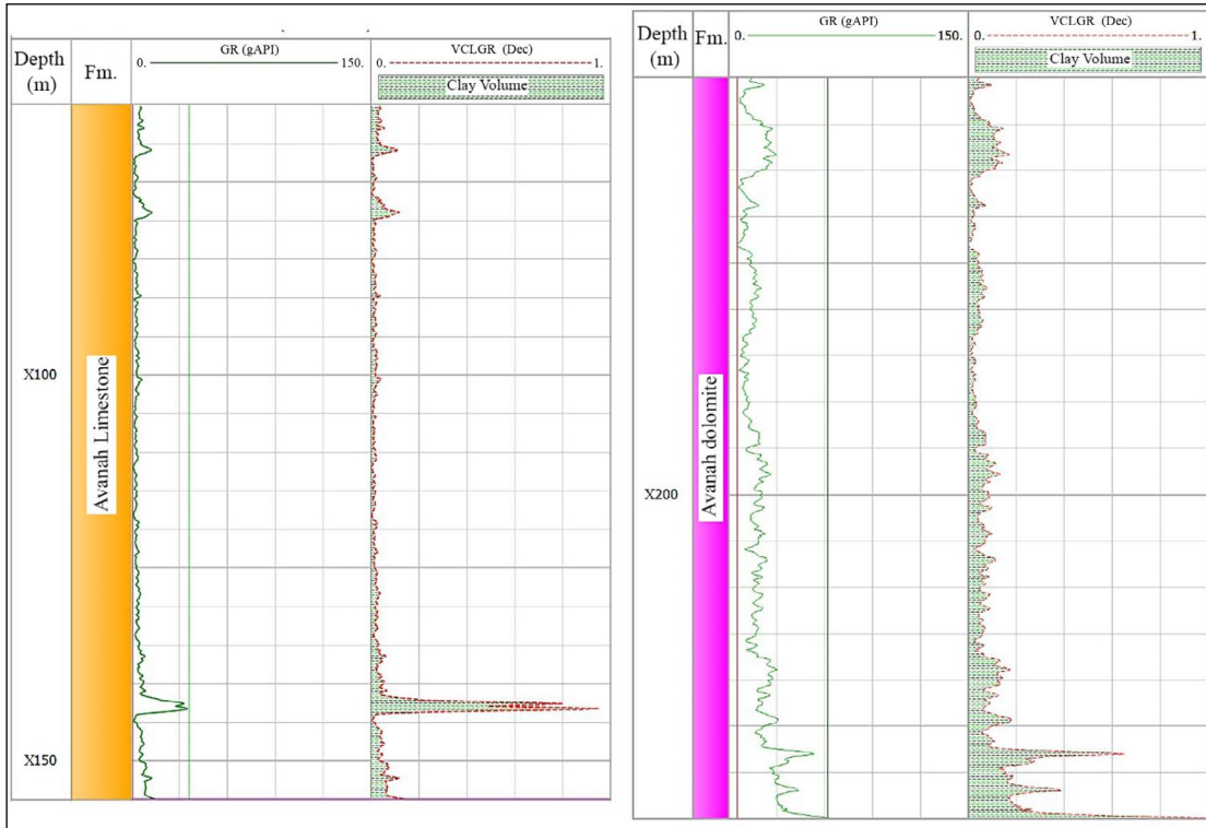
Figure 4- Clay volume within the both units of the studied Avanah Formation.
