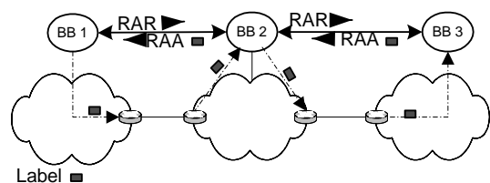
Figure 4. BB Signaling and label distribution.
