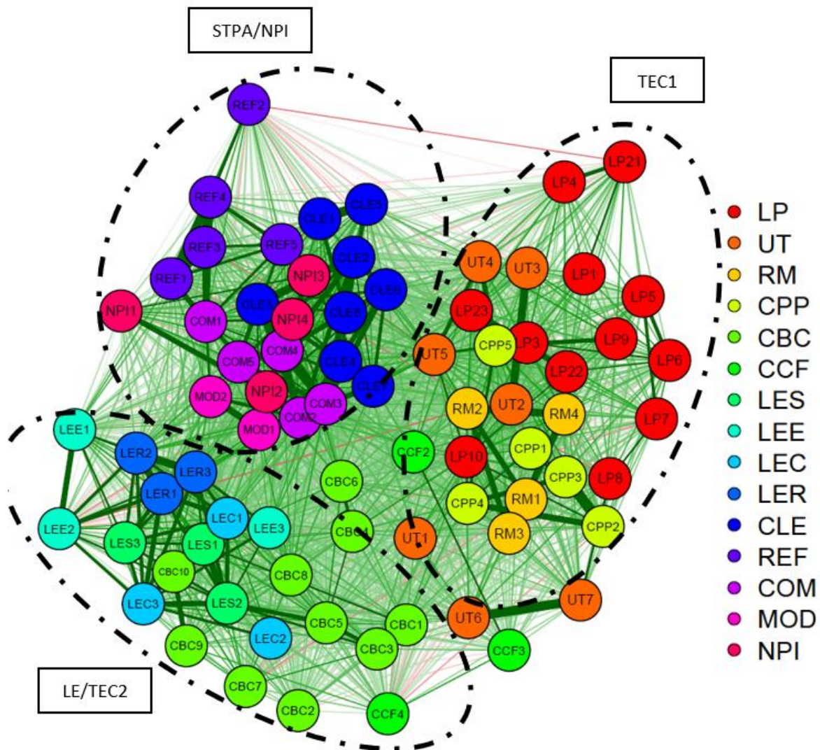
Figure 4. The network generated by all the scales' items for the Intermediate group ( n = 104 ), with three clusters still somewhat separated but more intermeshed: STPA/NPI, TEC1, and LE/TEC2.
