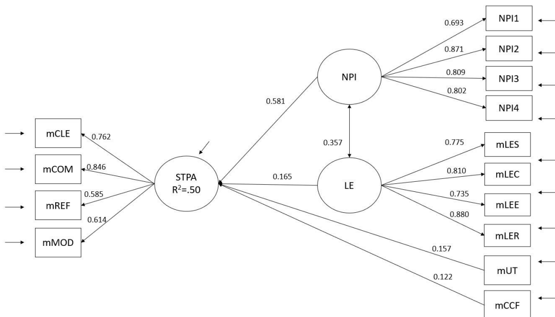
Figure 1. The interrelations between components of STPA, NPI, LE, mUT, and mCCF for the whole sample of students. (Standardized model: \chi^2(41, N = 283) = 242.22, p = .0081 ; CFI/TLI = .97/.97; RMSEA = .04, 95% CI [.02, .05].)
