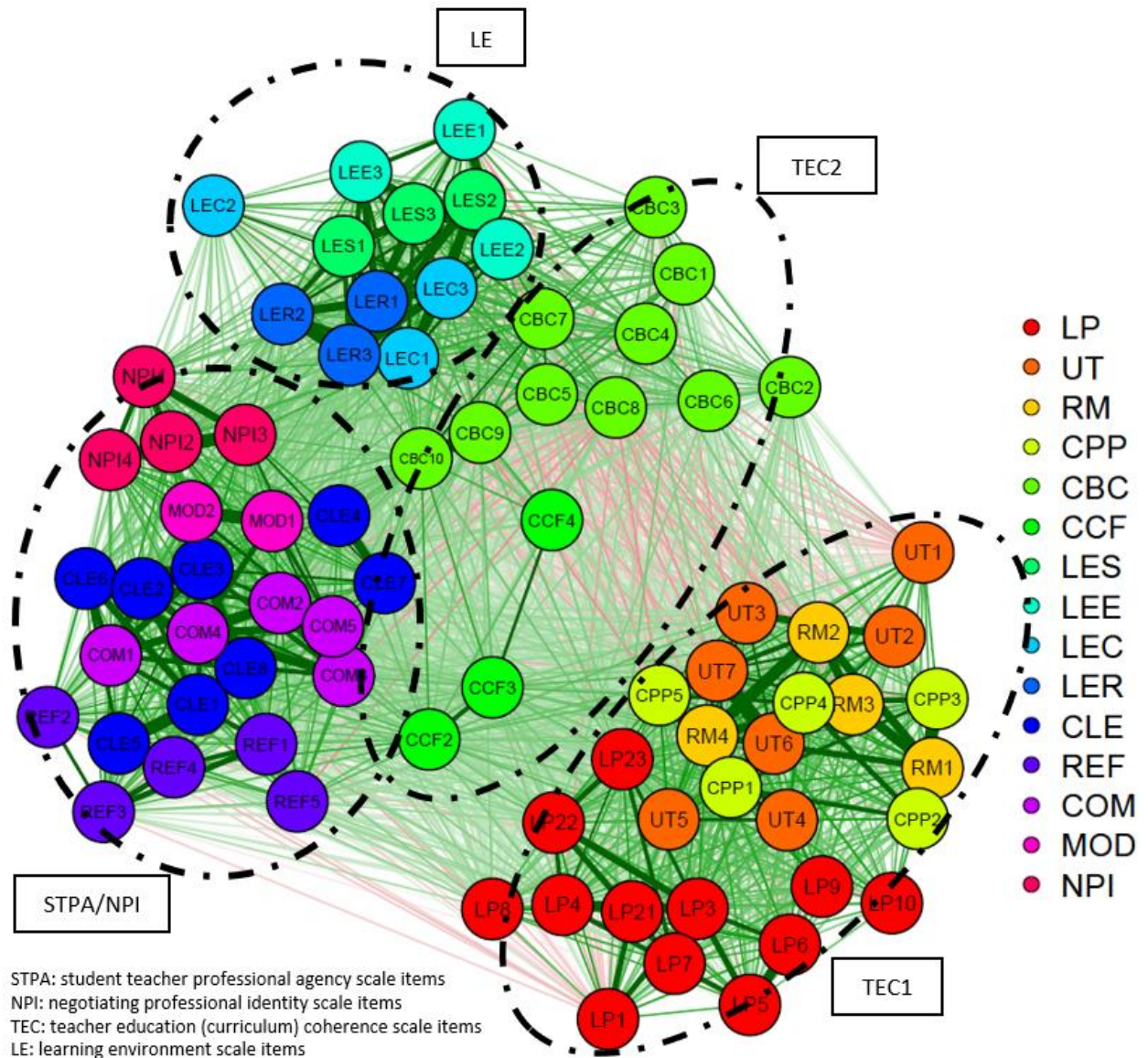
Figure 3. The network generated by all the scales' items for the Beginning group ( n = 145 ), with four clear clusters: STPA/NPI, TEC1 and TEC2, and LE.
