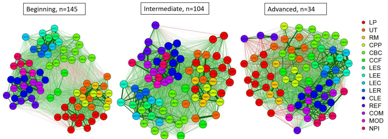
Figure 2. The networks generated by all the scales' items for the three groups of students: Beginning, Intermediate, and Advanced.
