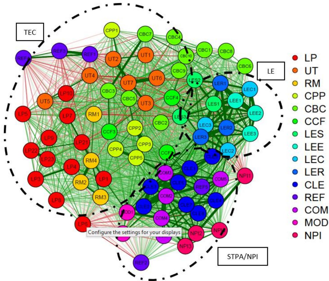
Figure 5. The global network generated by all the scales' items for the Advanced group ( n = 34 ).
