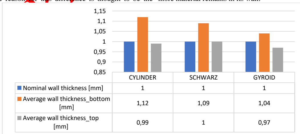
Figure 16. Average wall thickness measured from the bottom surface, average wall thickness measured from the top surface, nominal wall thickness measurements of all models
