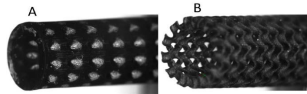
Figure 17. Schwarz model image (A) Gyroid model image (B)
