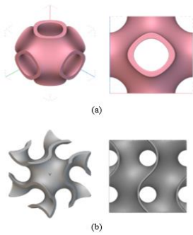
Figure 4. (a) Schwarz (b) Gyroid unit cells
