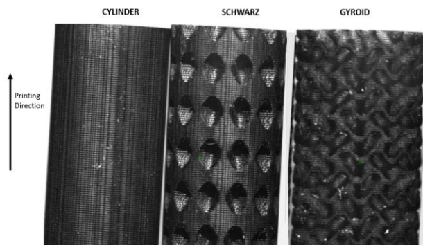
Figure 8. 3D printed TPMS based nerve guide conduits
