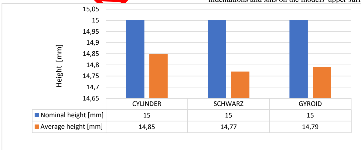
Figure 11. Nominal heights and measured average heights of the nerve guide conduit models determined during the design
