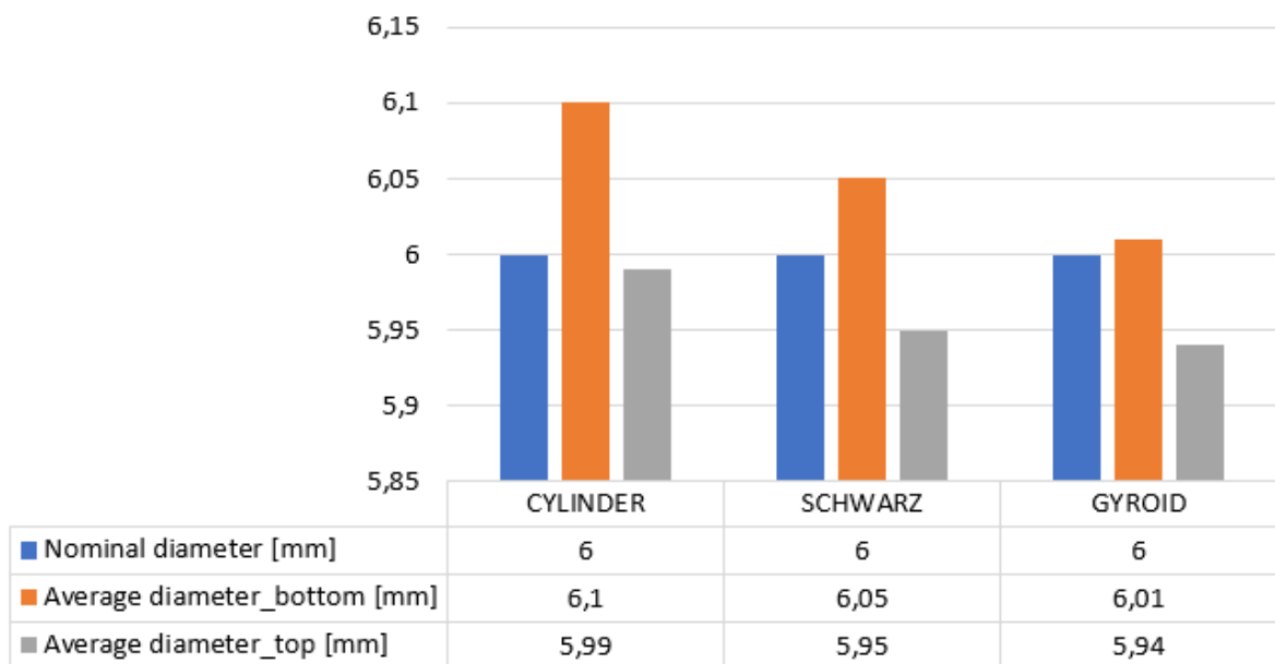
Figure 13. Average outer diameter measured from the lower surface, average outer diameter measured from the upper surface, nominal outer diameter dimensions of all models
