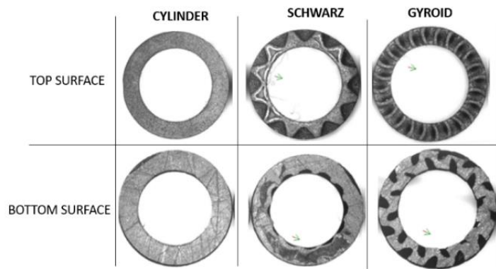
Figure 15. Bottom and top surface images of the produced nerve guide conduits
