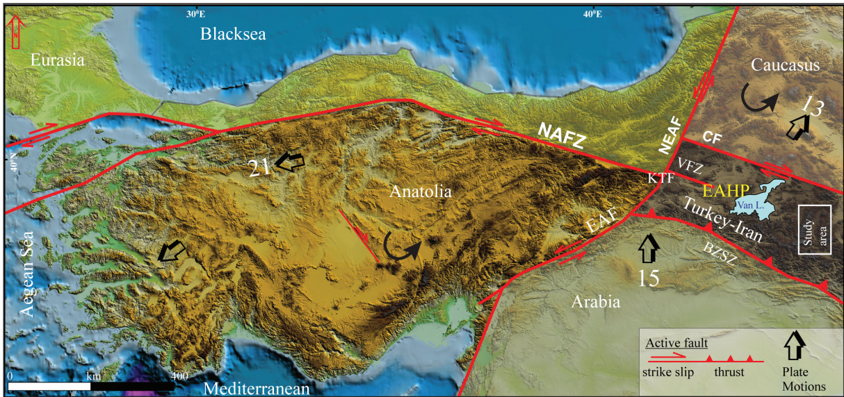
Figure 1- Location of the study area within Turkey's neotectonic framework (block boundaries taken from Reilinger et al., 2006; Djmour et al., 2011) (NAFZ: North Anatolia Fault Zone, EAFZ: East Anatolia Fault Zone, BZSZ: Bitlis-Zagros Suture Zone, CF: Çaldıran Fault, KTF: Karllova triple junction, VFZ: Varto Fault Zone, NEAF: Northeast Anatolia Fault, EACT: East Anatolia Compressional Tectonic block).
