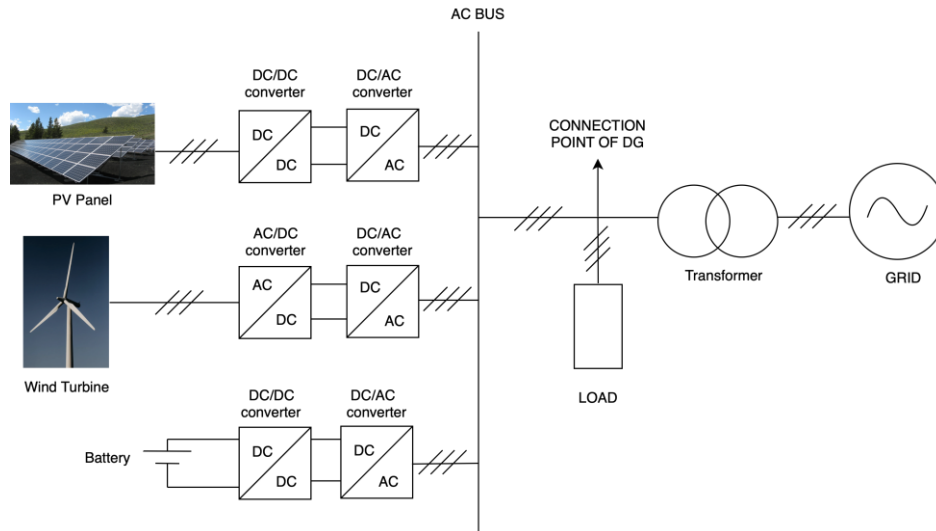
Figure 1. Grid-connected DG unit consisting of wind, solar and battery.
