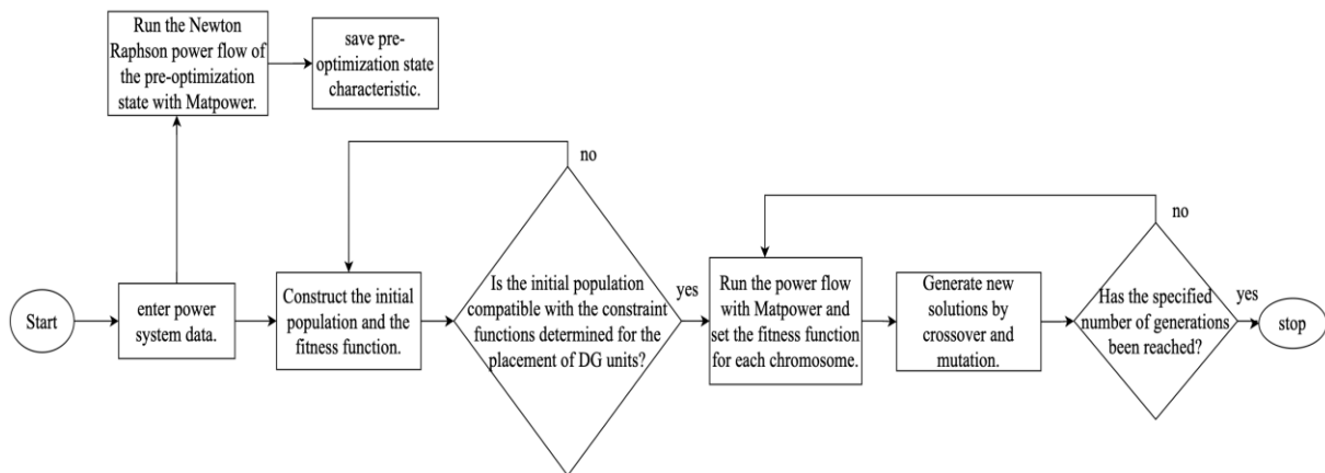
Figure. Flowchart of the proposed algorithm.
