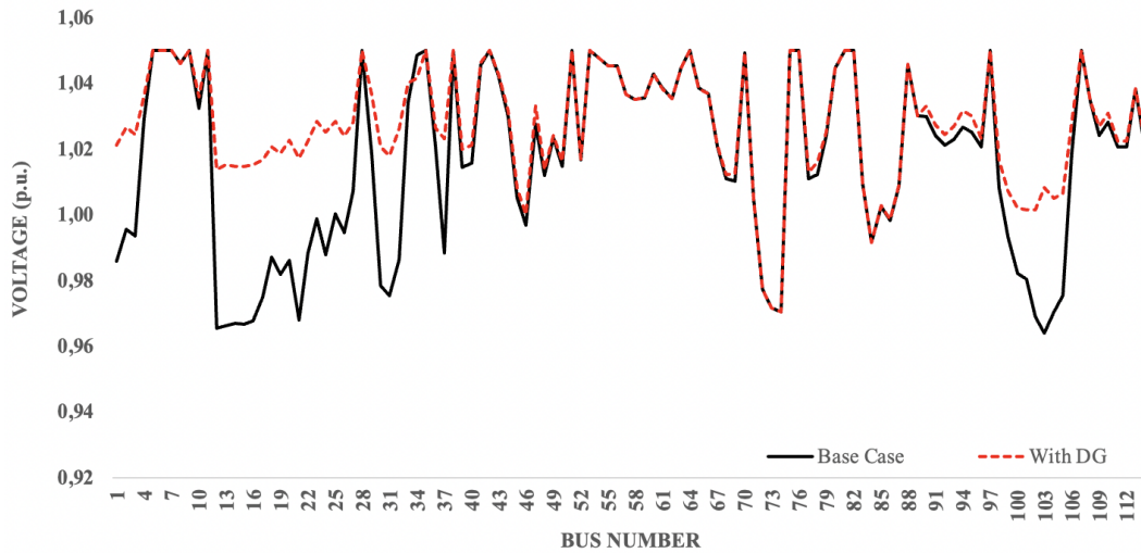
Figure 6. Voltage profile for Case.
