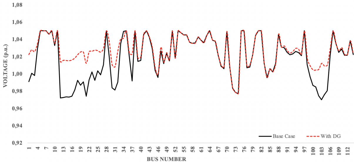
Figure 4. Voltage profile of Case 1.
