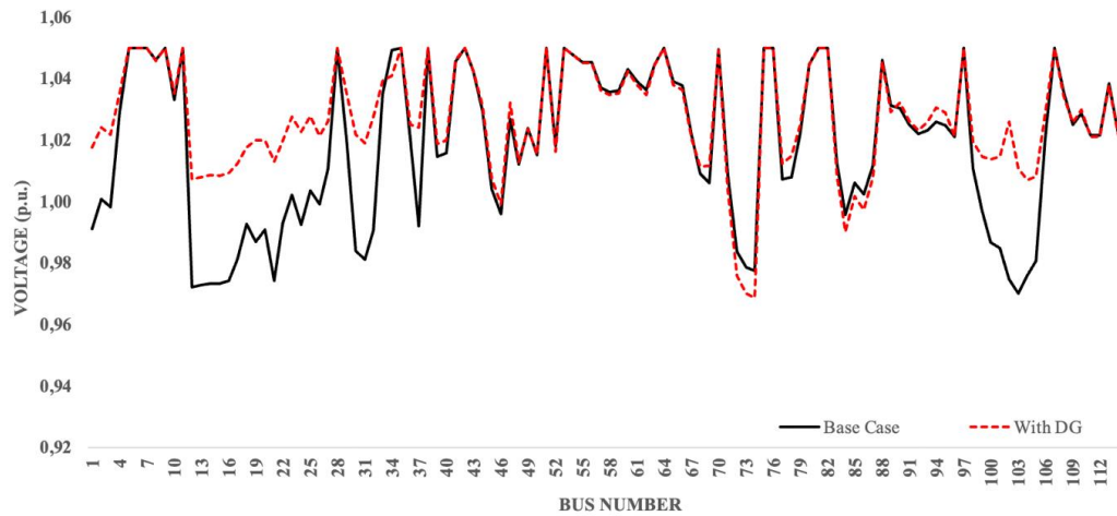
Figure 7. Voltage profile for Case 4.
