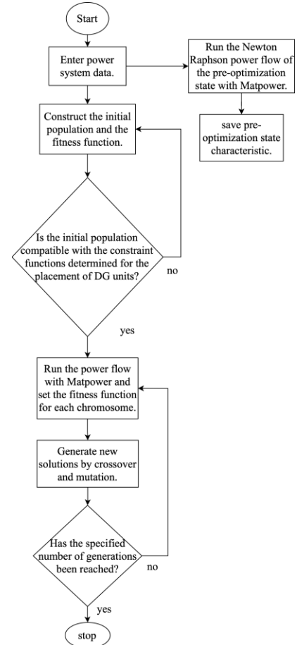
Figure 2. Flowchart of the proposed algorithm.
