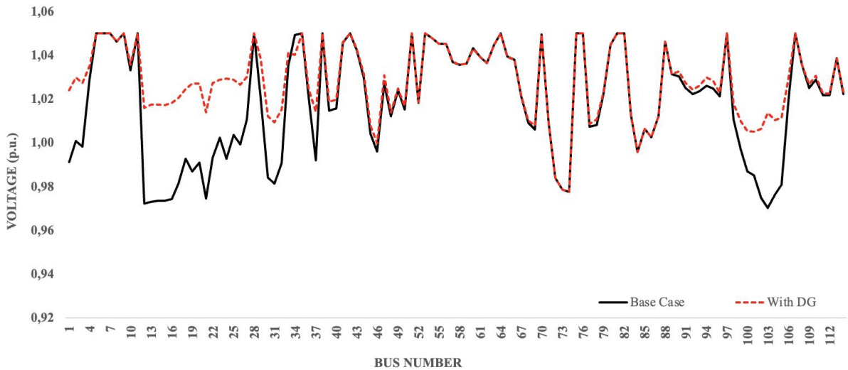
Figure 5. Voltage profile of Case 2.
