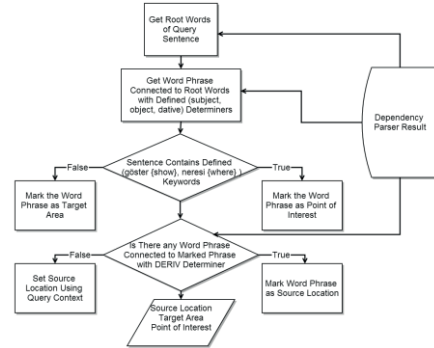
Figure 3: Parameter extraction process of the Map domain.
