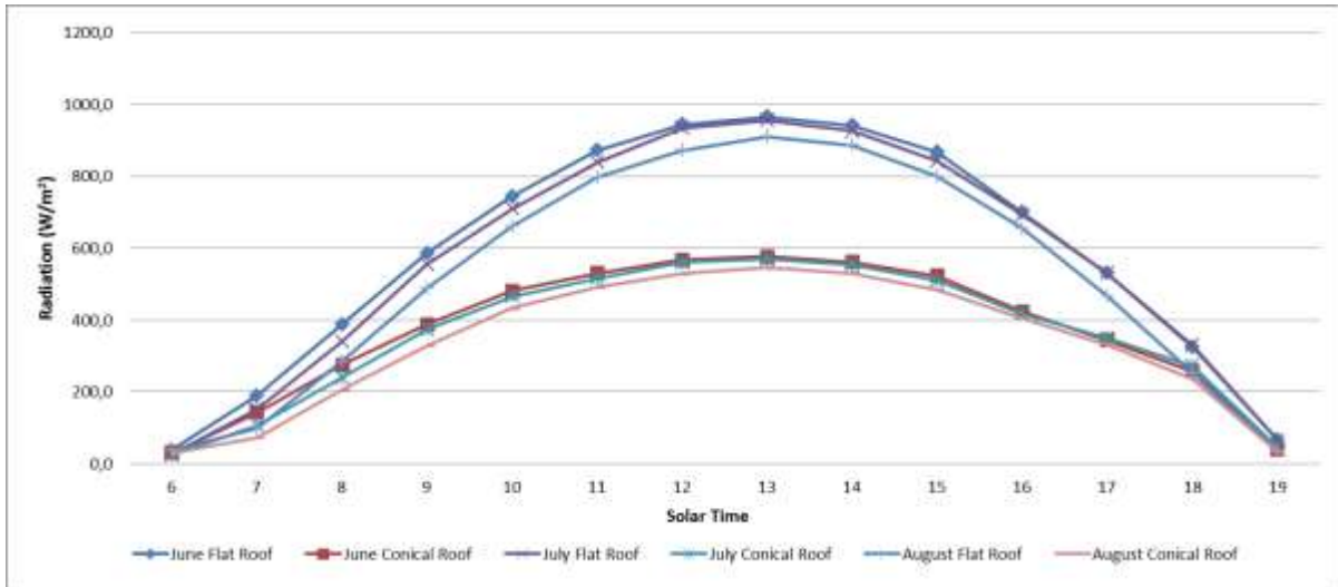
Figure 4. The average hourly solar radiation received by the unit area of the flat and conical roof for the summer months.
