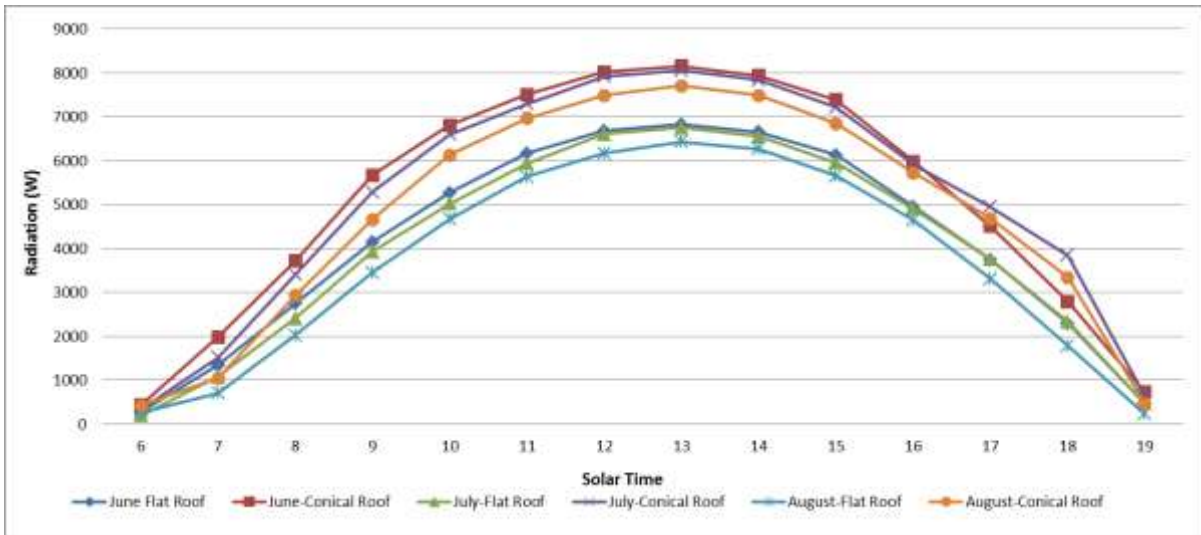
Figure 5. Hourly solar radiation on the conical roof Harran House ( \beta = 60^\circ ) and the flat surface has equivalent base area with conical roof house for the summer months.
