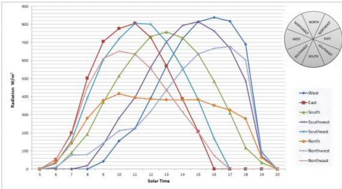
Figure 6. Variation of the solar radiation on the surface of the conical roof depending on surface azimuth angle during daylight, July, \beta = 60^\circ .
