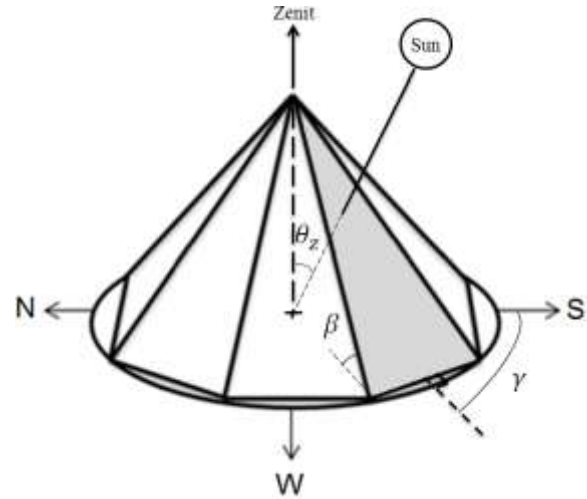
Figure 2. The simplified model of the conical roof and the essential angles for the solar geometry.
