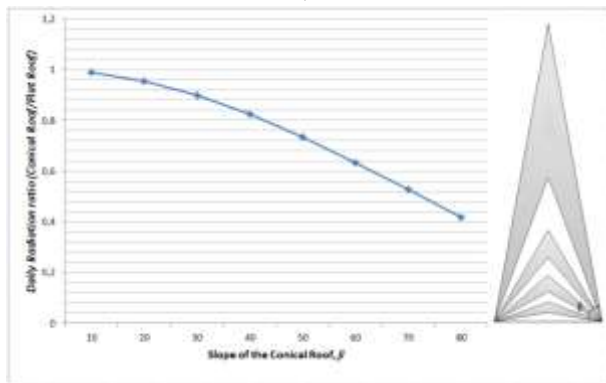
Figure 7. The ratio of the total daily radiation on a unit area of the conical roof for the different conical slope angles ( \beta changing from 10^\circ to 80^\circ ) to the total daily radiation on the unit area of the flat roof
