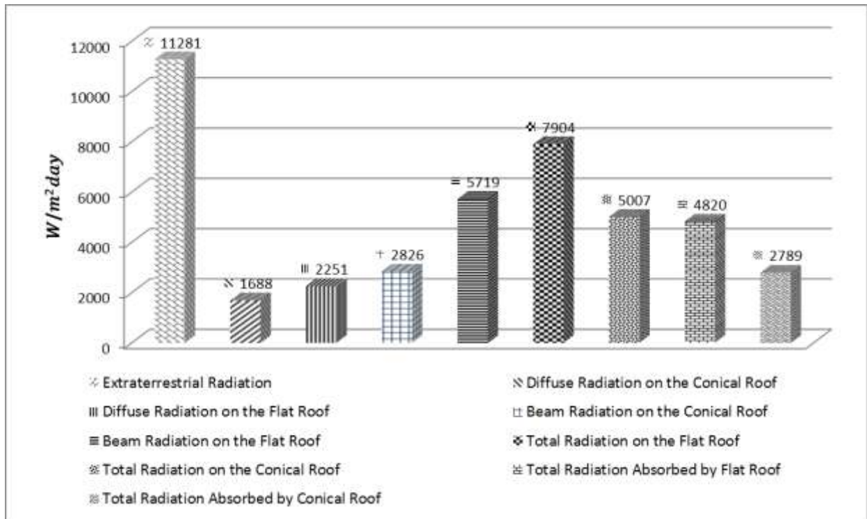
Figure 8. Comparison of the daily extraterrestrial, total, beam, diffuse radiation received by the conical( \beta = 60^\circ ) and the flat roof.
