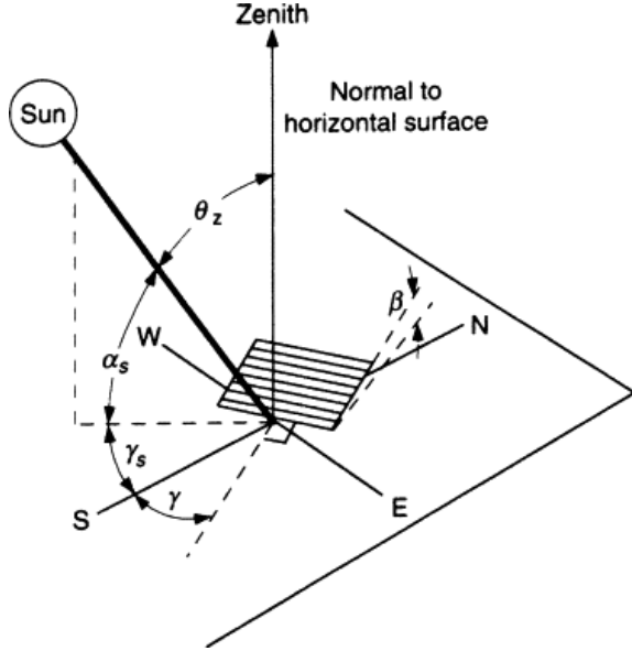
Figure 3. Zenith angle, slope, surface azimuth angle and solar azimuth angle for a tilted surface (Duffie and Beckman, 1991)
