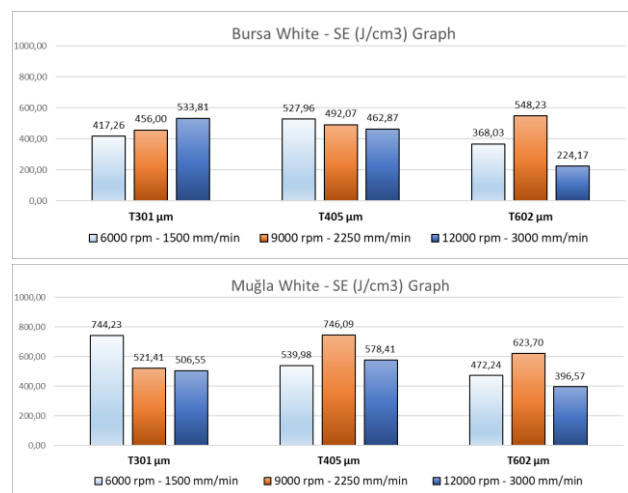
Figure 5. Spesific energy graphs
