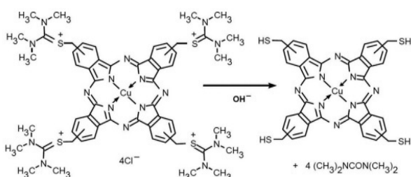
Figure 1. Structure of alcian blue 8G and its reaction with alkali to form an insoluble pigment (Scott 1972).
