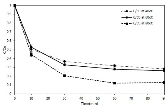
Figure 4. Decolorization of AB 8GX by Heat/Persulfate process at pH 5.7
