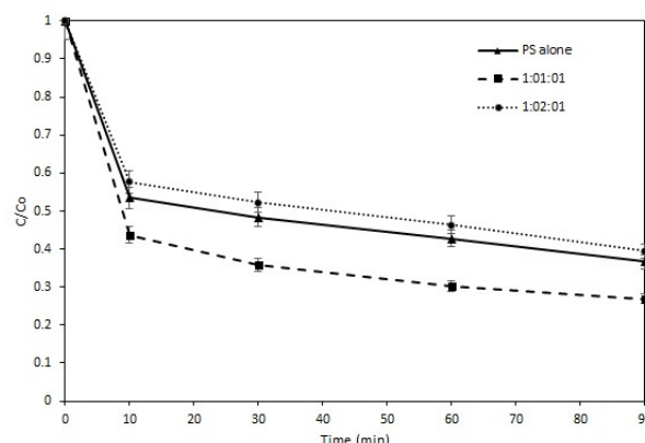
Figure 3. Decolorization of AB 8GX at pH 3 by Fe 2+ /Persulfate
