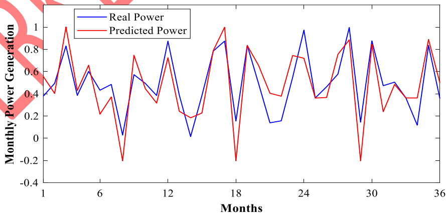
Figure 8. Test graph of the LSTM-SVR model with 11 parameters (11 parametrelı LSTM-SVR modelinin test grafiđi)
