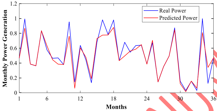
Figure 6. Test graph of the SVR model with 11 parameters (11 parametrelı SVR modelinin test grafiđi)
