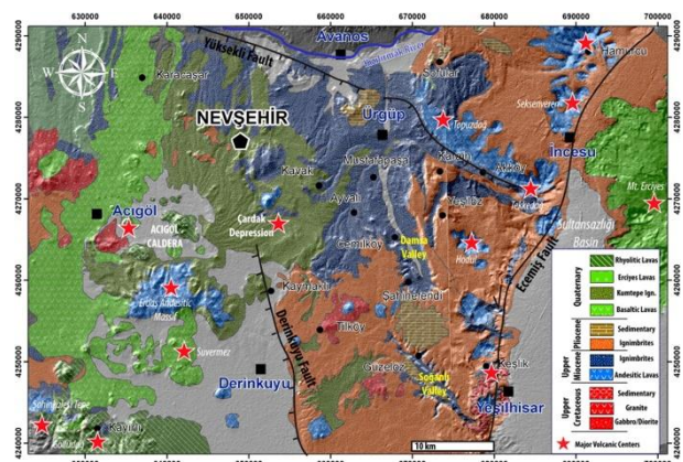
Figure 1. Geological map of Nevsehir region and distribution of pyroclastic deposits [21]
