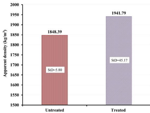
Figure 9. Change in apparent density ( \text{kg/m}^3 ) values of untreated and epoxy coated (treated) ignimbrite samples (StD: standard deviation)
