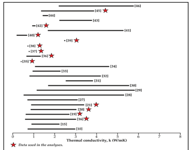
Figure 1. Different k values for various natural stones documented in previous literature.
