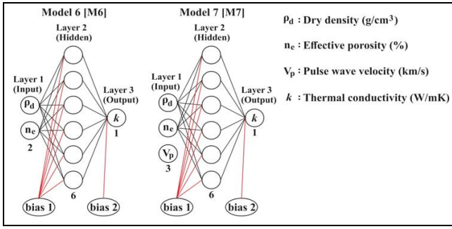
Figure 2. ANN structures considered in this study.
