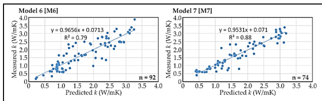
Figure 4. Predicted and measured k values for the ANN-based models (M6-M7).
