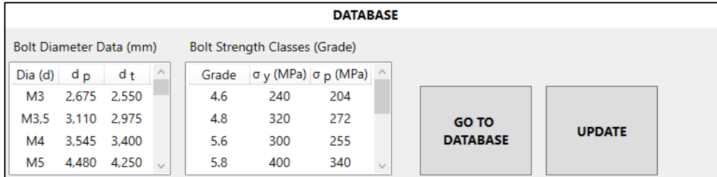
Figure 8. Database
