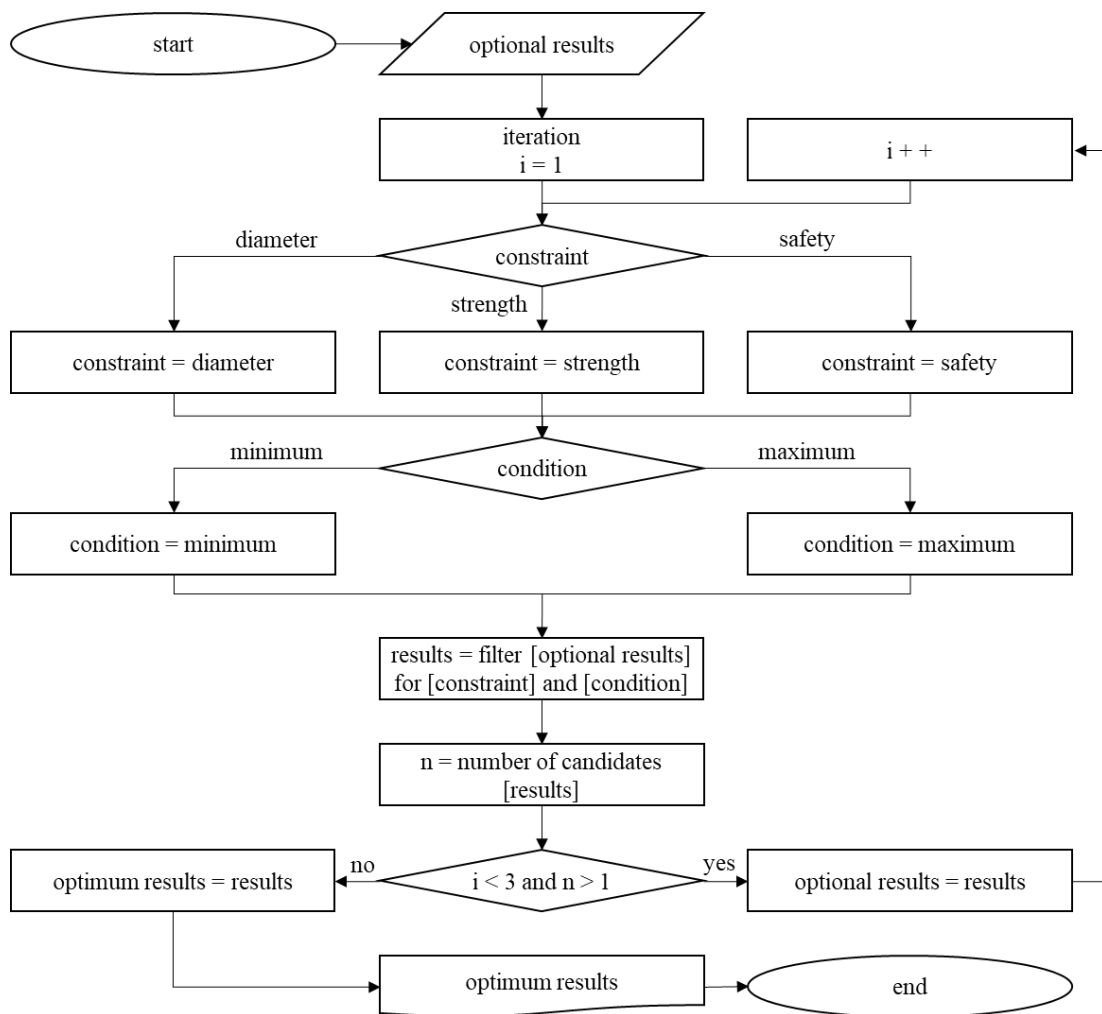
Figure 13. Optimization algorithm
