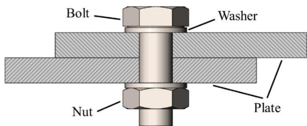
Figure 1. Bolted joint
