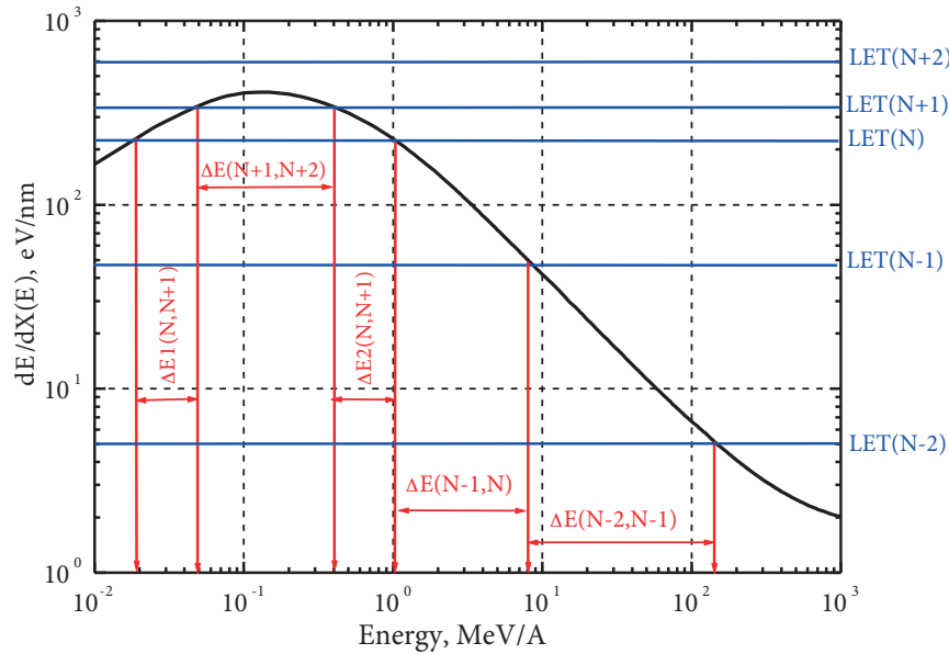
Figure 2. Layout of LET and corresponding energy intervals \Delta E on the curve dE/dX(E) .
