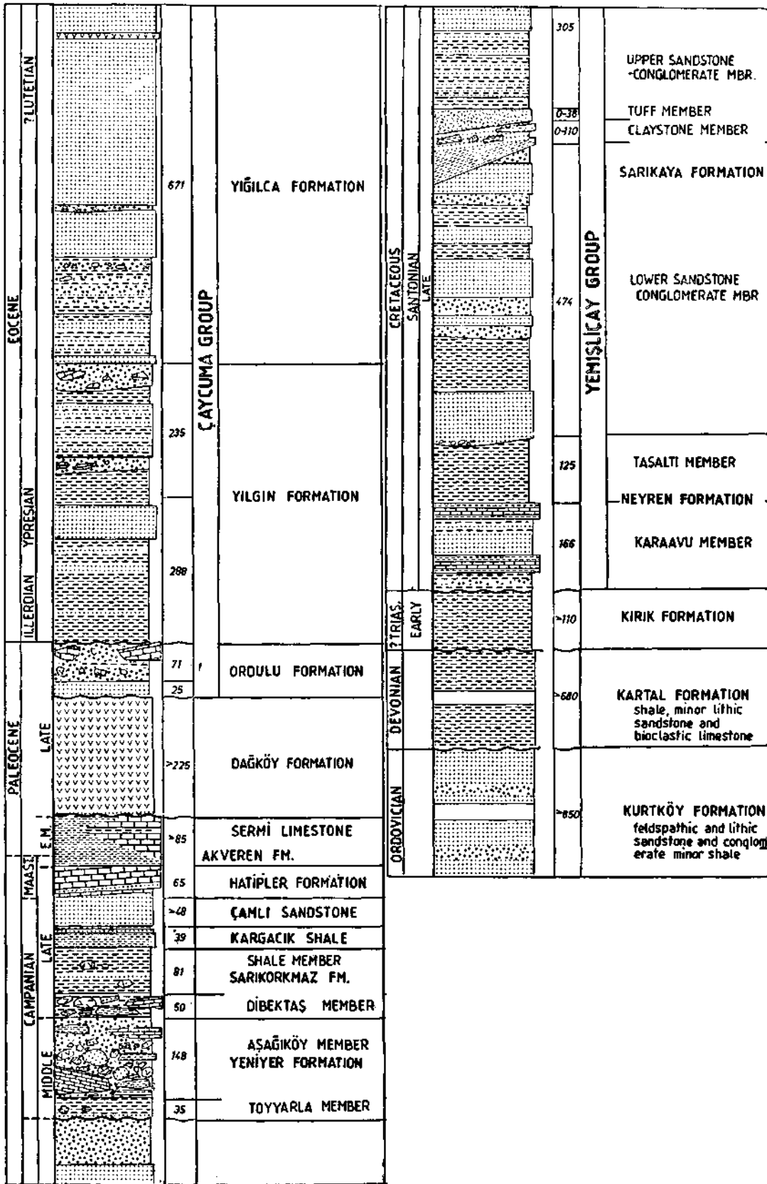
Fig. 3 - Generalized rock succession of the Yiğilca area. The Paleozoic and older rocks (Kaya, 1982) have not been dealt with in this study.
