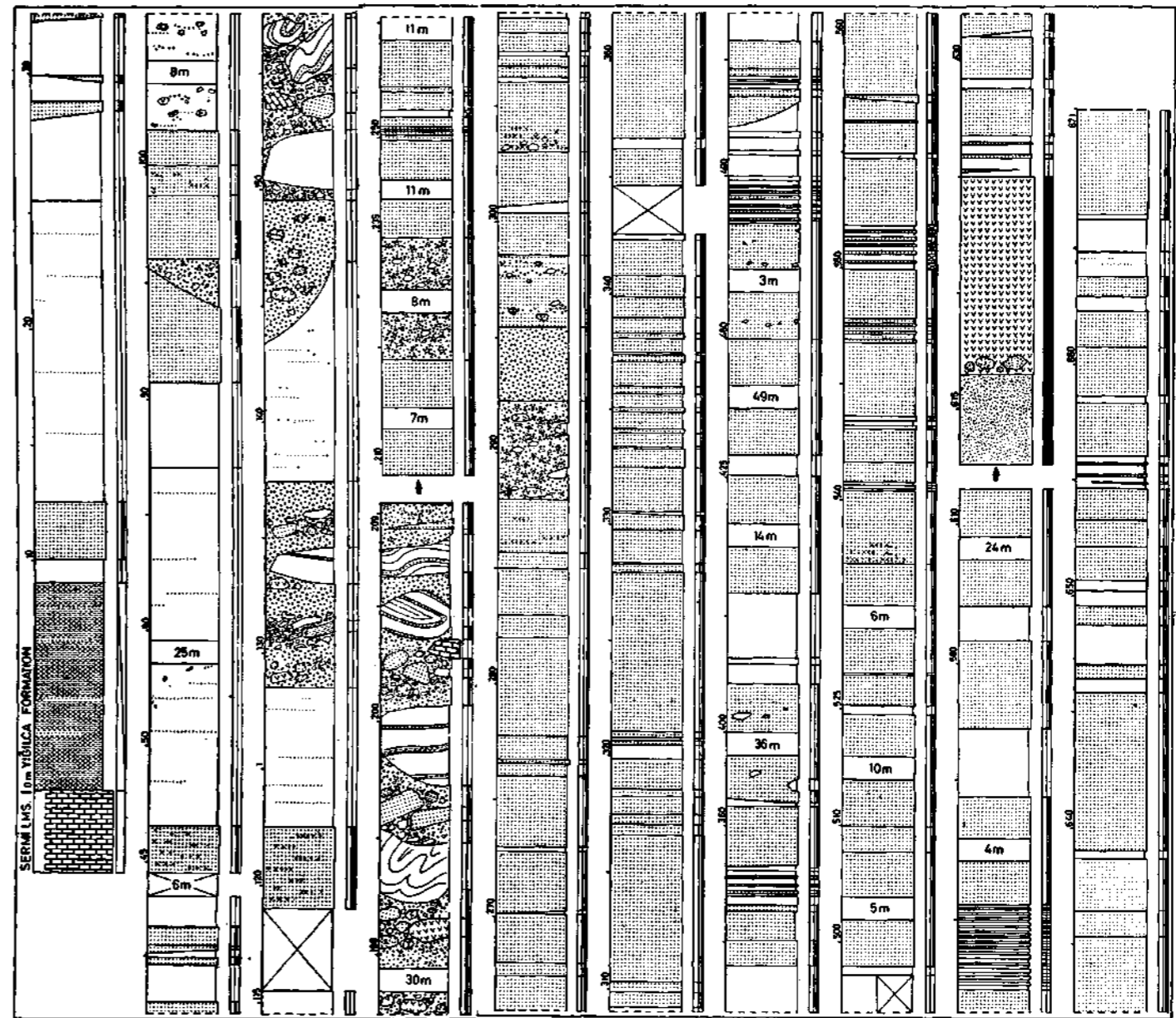
Fig. 11 - Partial composite type section of the Yigilca formation.
