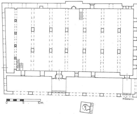
Figure 2. Ulu Mosque and Minaret ground floor plan (Gönültaş, 2018)
