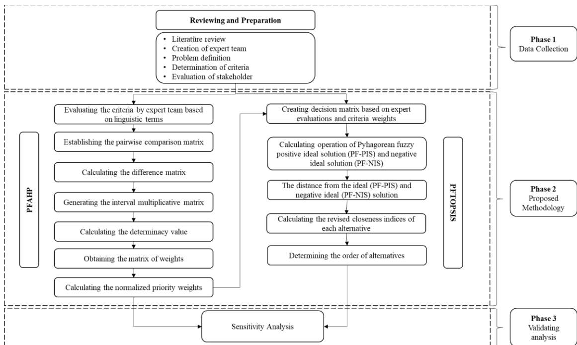
Figure 3. Application flow
