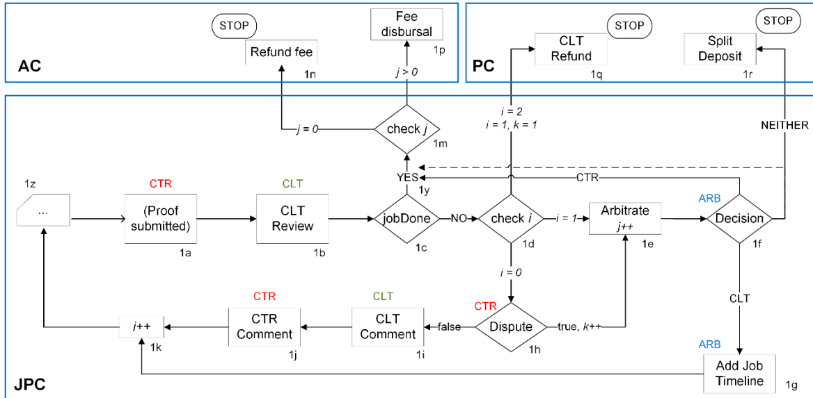
Fig. 4. Scenario #1 major process interactions (adapted from Fukuzawa (2024)).
