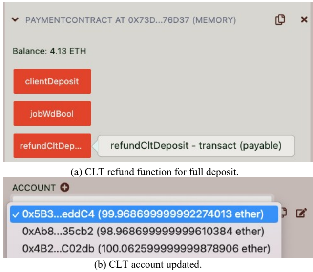
Fig. 12. Process of full CLT refund after arbitration ruling (adapted from Fukuzawa (2024)).
