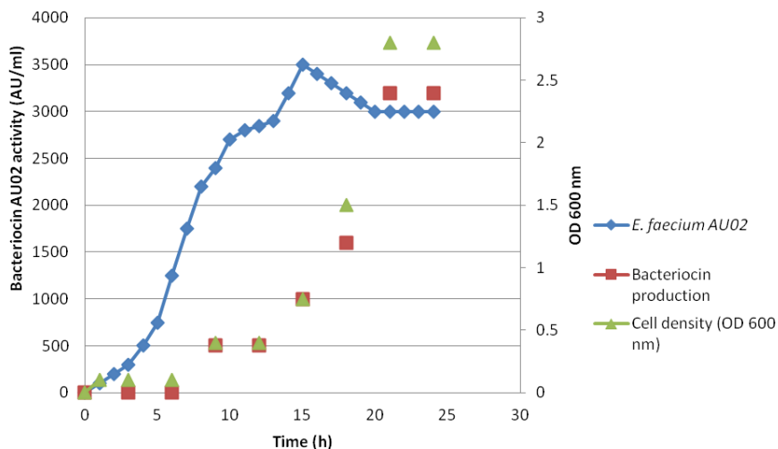
Figure 3. Growth of E. faecium AU02 in MRS broth in association with bacteriocin production at different cell densities.
