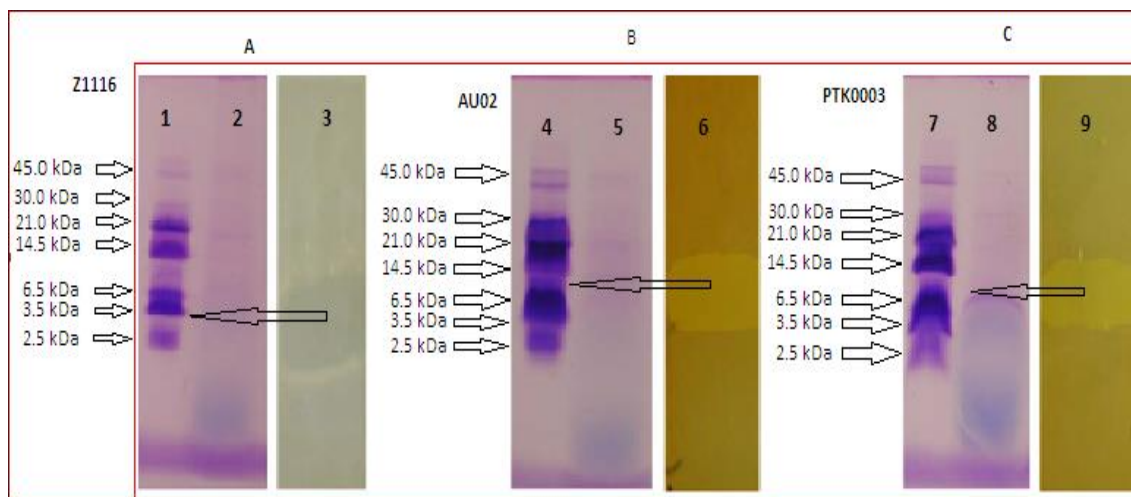
Figure 5: Tricine-SDS-PAGE of bacteriocins Z1116, AU02 and PKT0003. Lanes 1, 4 and 7: molecular mass marker (2.5–45.0 kDa, Amersham). Lanes 2, 5 and 8: peptide bands stained with Coomassie Blue R250. Lanes 3, 6 and 9: zones of growth inhibition corresponding to the position of bacteriocins Z1116, AU02 and PKT0003, respectively. The gel was overlaid with E. faecium HKLHS and L. sakei DSM 20017, respectively (ca. 1 \times 10^6 CFU/ml) suspended in BHI and MRS agar. The sizes of bacteriocins Z1116, AU02 and PKT0003, as revealed by tricine-SDS-PAGE, were 3.2 kDa, 10 kDa and 10 kDa, respectively.
