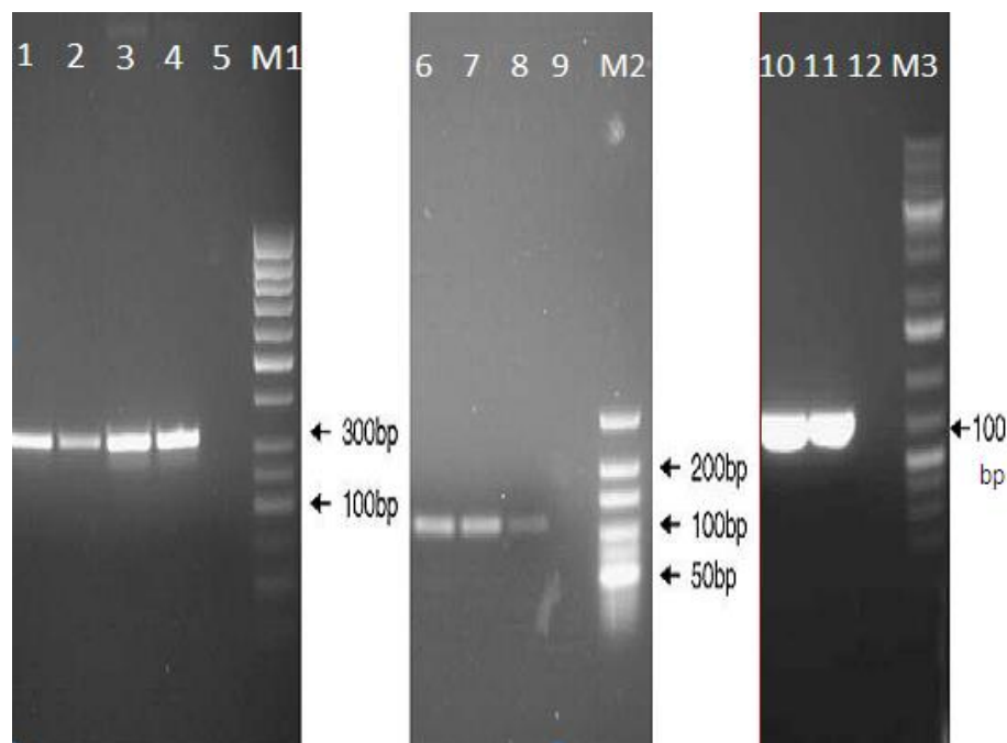
Figure 1: Agarose gels showing DNA fragments obtained after PCR with species-specific and genus-specific primers. Lanes 1 and 2: strain Z1116, lanes 3 and 4: L. plantarum NCBF 363, lane 5: no DNA loaded, lane M1: O'GeneRuler™ 100-bp DNA Ladder from Fermentas, lanes 6 and 7: strain AU02, lane 8: E. faecalis PTA-7278 (ST4SA), lane 9: no DNA loaded, lane M2:
