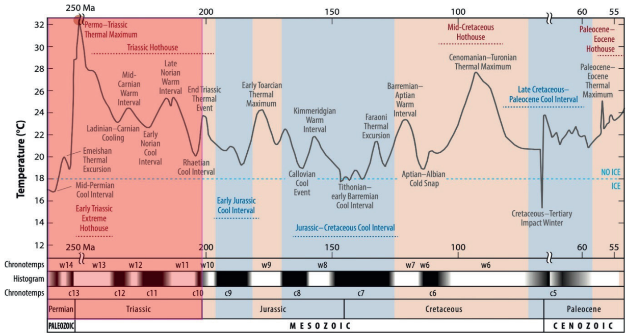
Figure 23. Mesozoic paleotemperature timescale showing warm intervals (white) and cool intervals (black). During the Early Triassic, global temperatures reached extreme hothouse conditions of \sim 32^{\circ}\text{C} , subsequently decreasing to \sim 24^{\circ}\text{C} by the Late Triassic. The Early–Late Triassic interval contains two warm and three cool phases. Following the Rhaetian, temperatures rose from \sim 19^{\circ}\text{C} to \sim 24^{\circ}\text{C} during the end-Triassic thermal event. The solid grey curve represents the Global Average Temperature, while the chronostratigraphic framework follows the International Chronostratigraphic Chart (2020/01) (Figure adapted from Scotese et al. (2021)).
