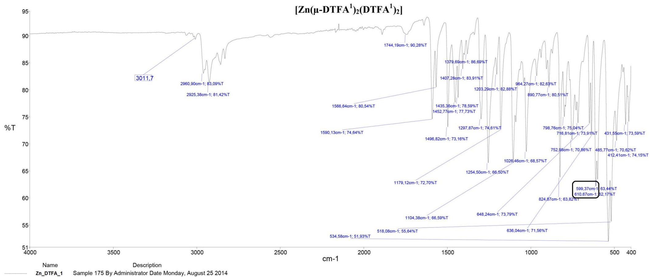
Scheme 1b. IR spectrum of [Zn( \mu -DTFA 1 ) 2 (DTFA 1 ) 2 ] (4000-400 cm -1 ).
