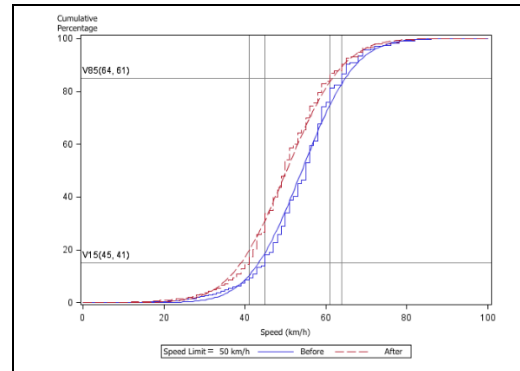
Figure 12. 'before'/'after' cumulative speed distribution and 85 th percentile speeds (sections with 50 km/h speed limit).
