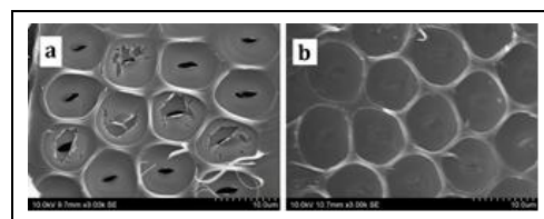
Figure 7. Representative SEM photographs of micro-explosion-treated. (a): and untreated. (b): Poplar samples. Source [35].
