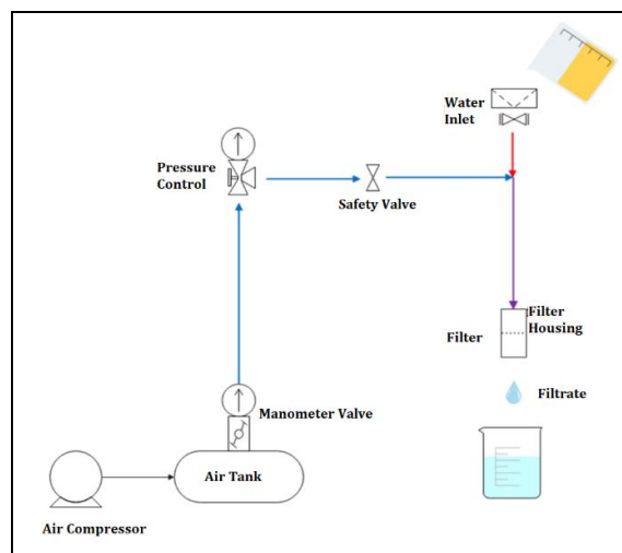
Figure 1. Schematic diagram of the filtration module and test system.
