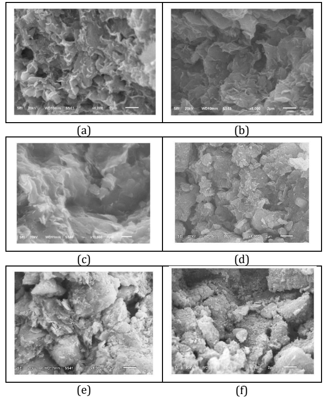
Figure 7. Fabric changes of the high plasticity samples. (a): Prepared with pure water and (b): 1M NaCl solution and (c): 1M CaCl 2 solution added (12,5kPa load stage); low plasticity samples. (d): Prepared with pure water and (e): 1M NaCl solution and (f): 1M CaCl 2 solution added (12.5kPa load stage).
