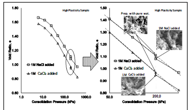
Figure 9. Osmotic effect of leaking salt solutions on void ratio-vertical stress ( e - \log p ) graphs and clay fabric (200kPa load range).
