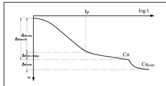
Figure 1. Appearance of time dependent deformation obtained from experiments for osmotic compression.
