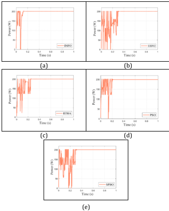
Figure 7. Results of shading 2 power- time graph. (a): INFO. (b): EEFO. (c): RTHA. (d): SPBO. (e): PSO.
