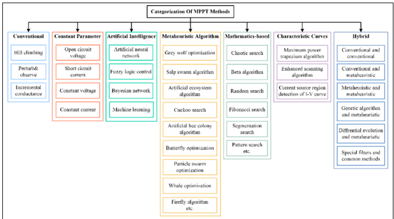
Figure 1. Categorization of MPPT methods.
