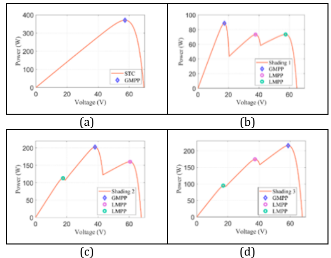
Figure 5. P-V curves under partial shading conditions. (a): STC. (b): Shading 1. (c): Shading 2. (d): Shading 3.
