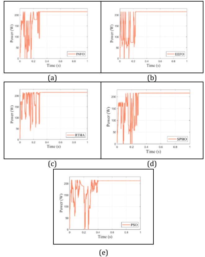
Figure 8. Results of shading 3 power- time graph. (a): INFO. (b): EEFO. (c): RTHA. (d): SPBO. (e): PSO.
