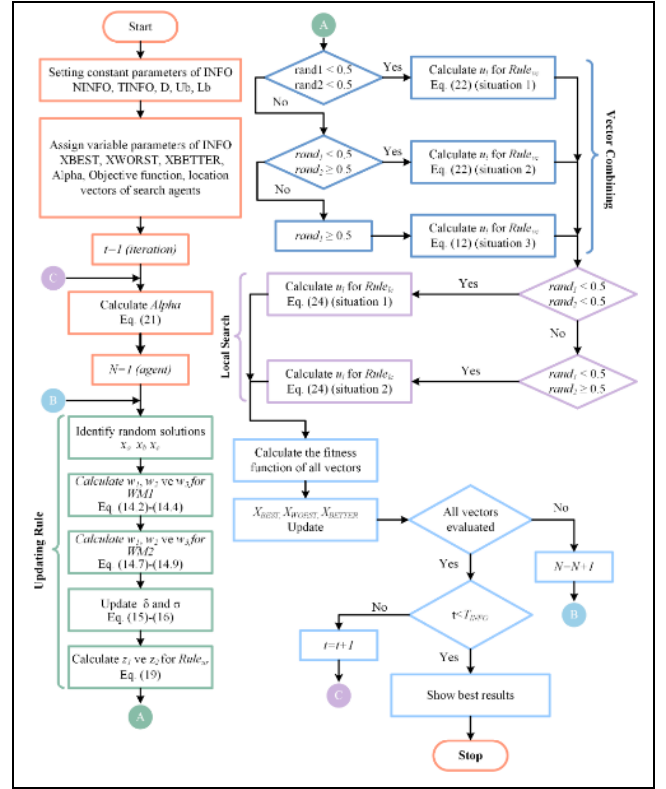
Figure 4. Flow diagram of the INFO algorithm
