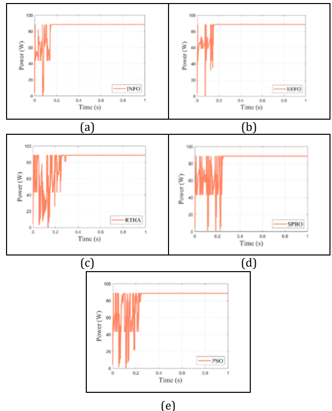
Figure 7. Results of shading 1 power-time graph. (a): INFO. (b): EEFO. (c): RTHA. (d): SPBO. (e): PSO.
