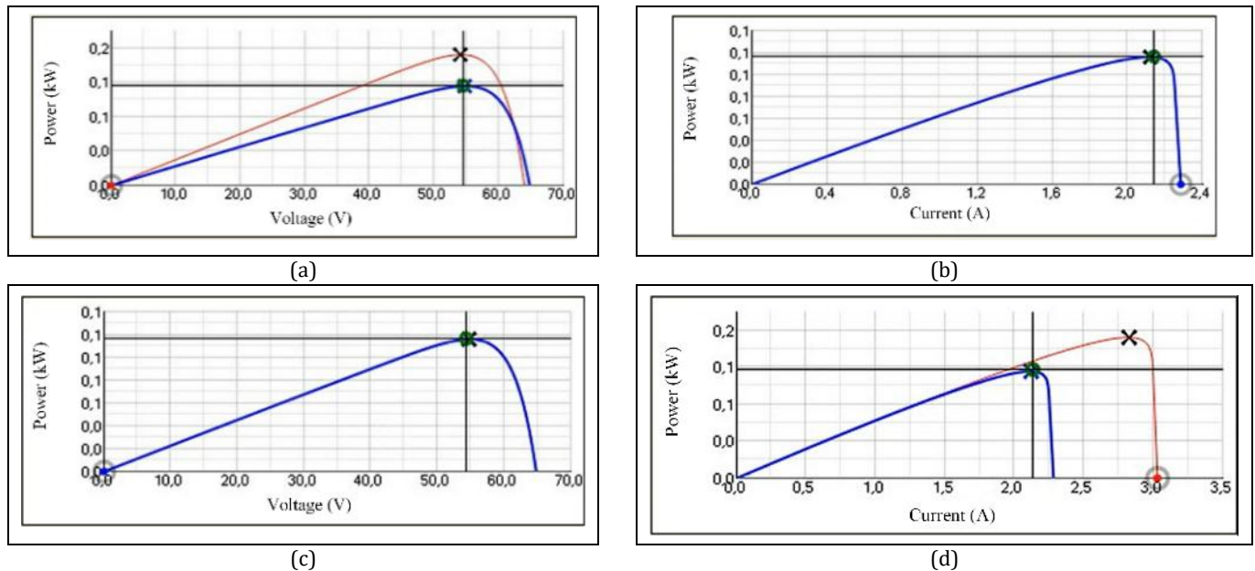
Figure 11. Experimental performance of the INFO algorithm: P-V and P-I profiles. (a): P-V curve at Test 1. (b): (b) P-I curve at Test 1. (c): P-V curve at Test 2. (d): P-I curve at Test 2.
