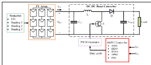
Figure 2. PV system and component.
