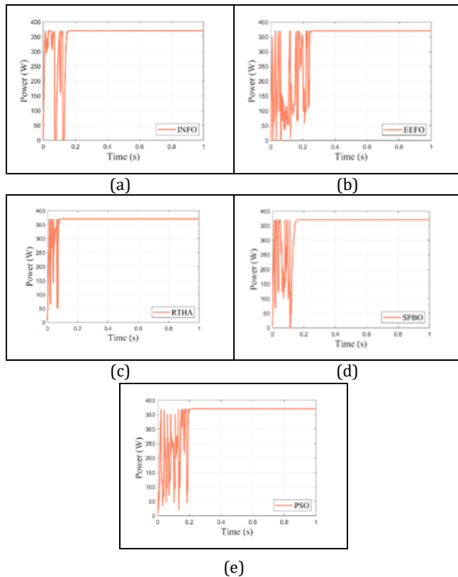
Figure 6. Results of the STC power-time graph. (a): INFO. (b): EEFO. (c): RTHA. (d): SPBO. (e): PSO.
