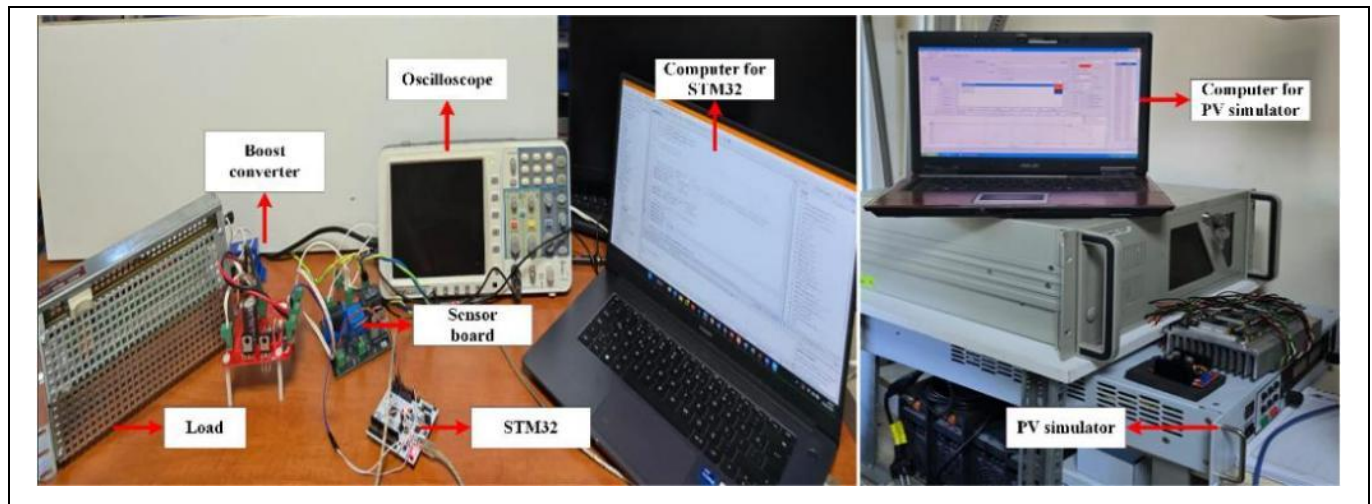
Figure 9. Experimental setup.
